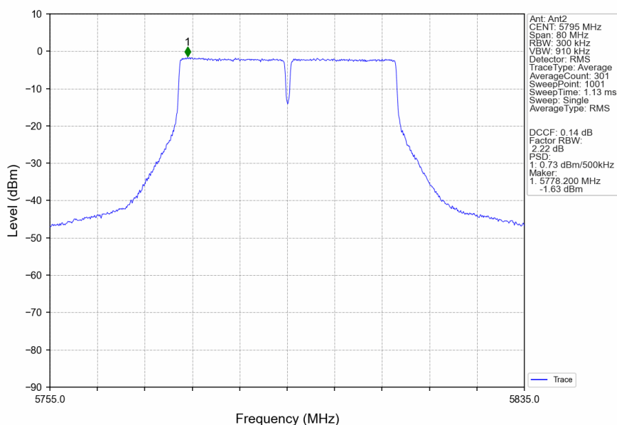
802.11ac(VHT40)_HCH_5795MHz_Ant2_NTNV
