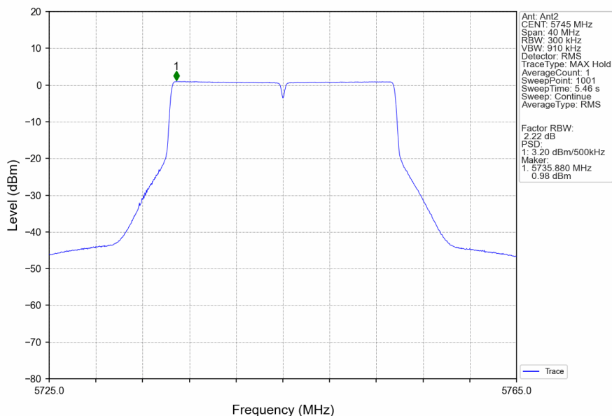
802.11ax(HEW20)_LCH_5745MHz_RU242_Left_Ant2_NTNV
