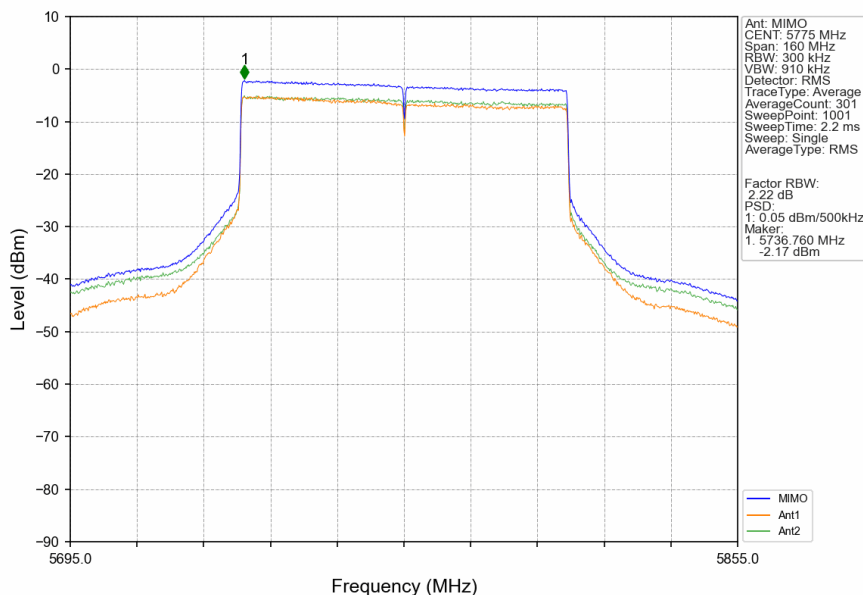
802.11ax(HEW80)_MCH_5775MHz_RU996_Left_MIMO_NTNV
