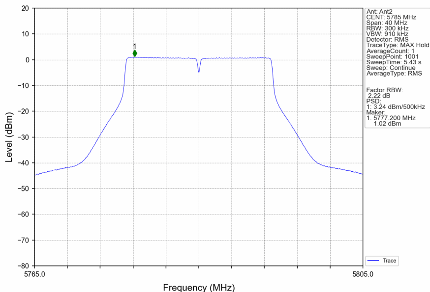
802.11n(HT20)_MCH_5785MHz_Ant2_NTNV
