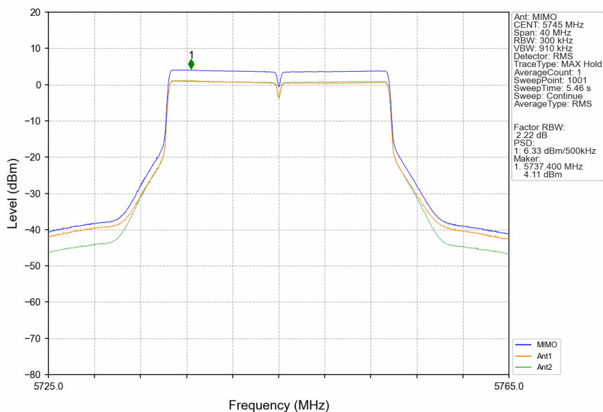
802.11ax(HEW20)_LCH_5745MHz_RU242_Left_MIMO_NTNV
