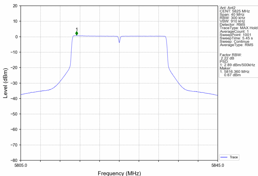
802.11ax(HEW20)_HCH_5825MHz_RU242_Left_Ant2_NTNV
