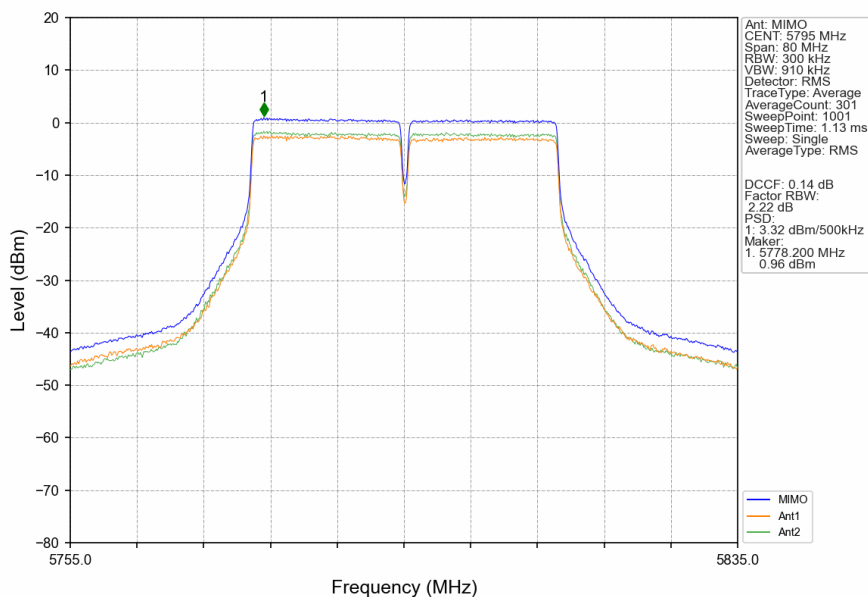
802.11ac(VHT40)_HCH_5795MHz_MIMO_NTNV
