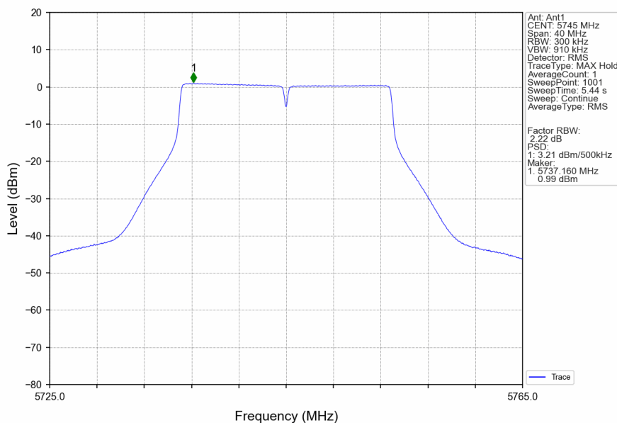
802.11ac(VHT20)_LCH_5745MHz_Ant1_NTNV
