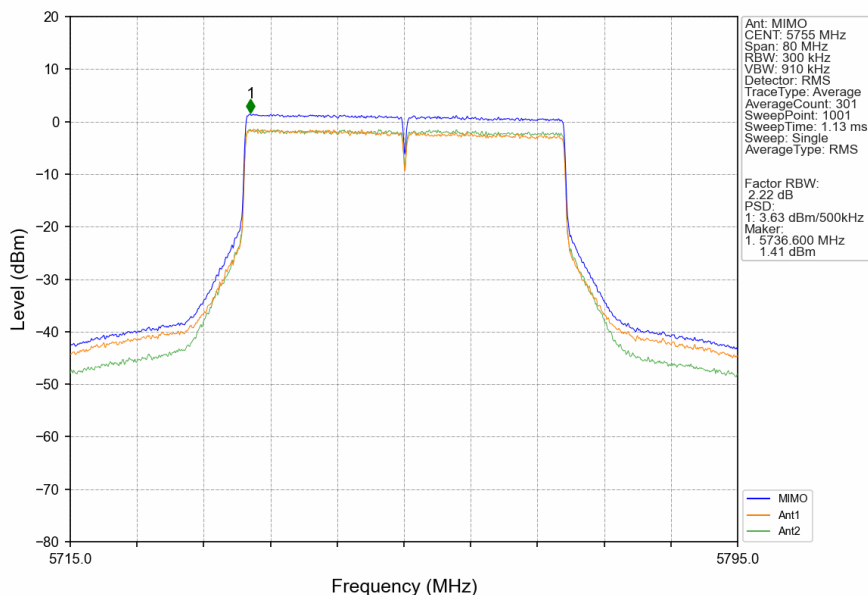
802.11ax(HEW40)_LCH_5755MHz_RU484_Left_MIMO_NTNV
