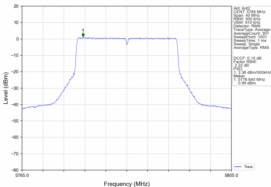
802.11ax(HEW20)_MCH_5785MHz_RU242_Left_Ant2_NTNV
