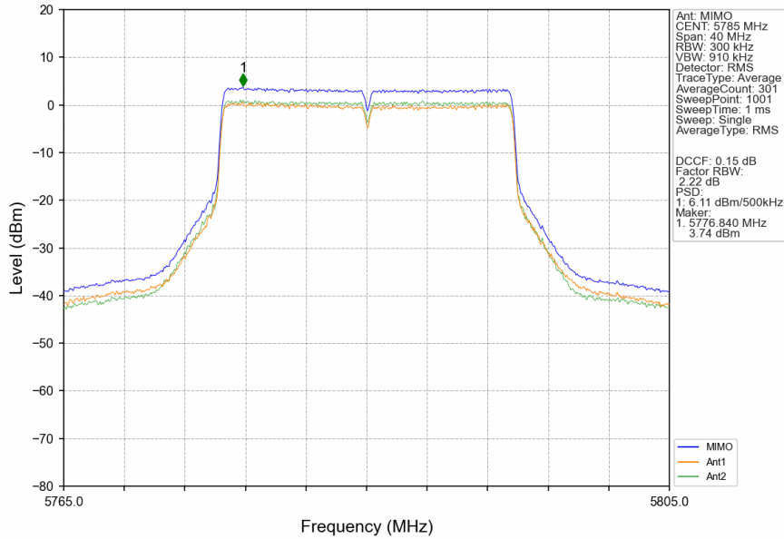
802.11ax(HEW20)_MCH_5785MHz_RU242_Left_MIMO_NTNV
