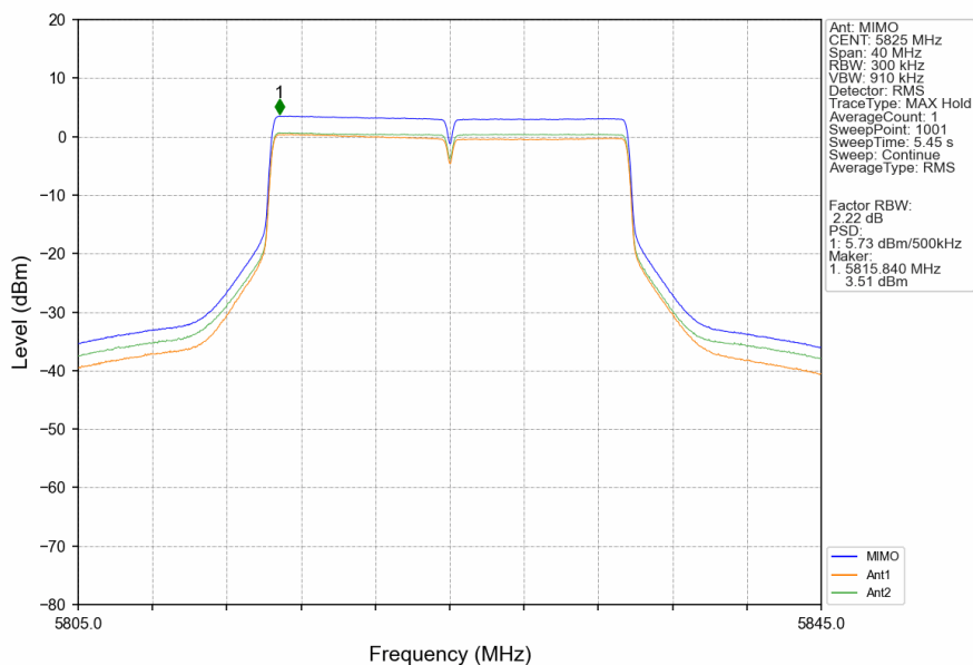
802.11ax(HEW20)_HCH_5825MHz_RU242_Left_MIMO_NTNV
