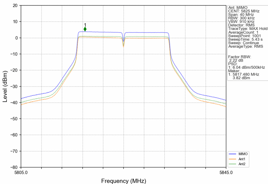
802.11ac(VHT20)_HCH_5825MHz_MIMO_NTNV
