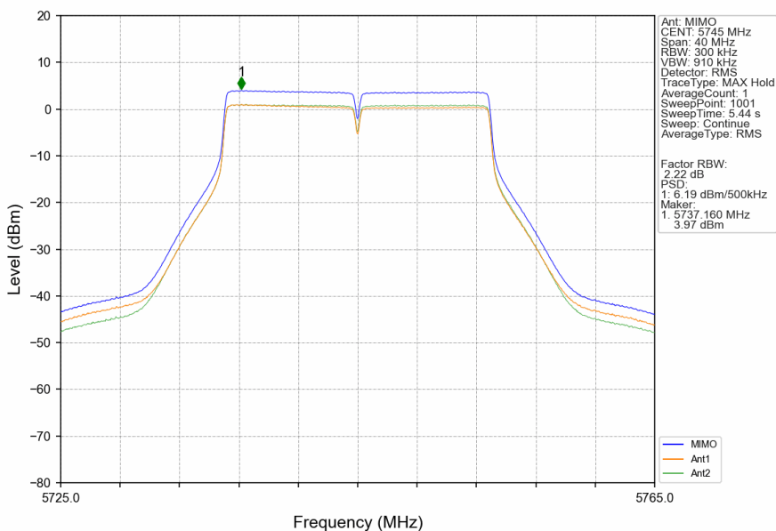
802.11ac(VHT20)_LCH_5745MHz_MIMO_NTNV
