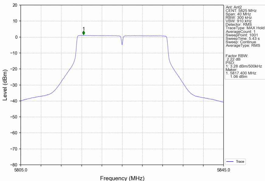
802.11ac(VHT20)_HCH_5825MHz_Ant2_NTNV
