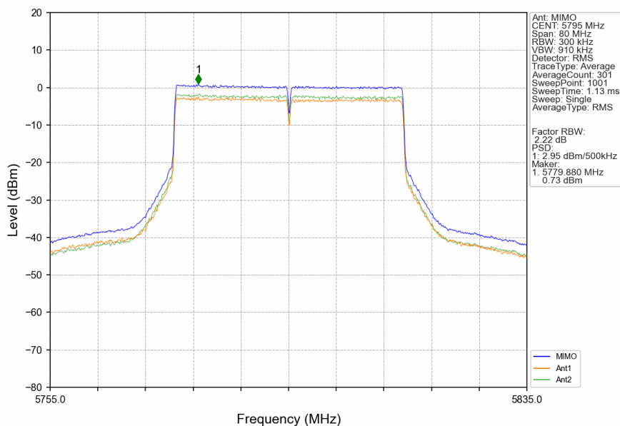
802.11ax(HEW40)_HCH_5795MHz_RU484_Left_MIMO_NTNV
