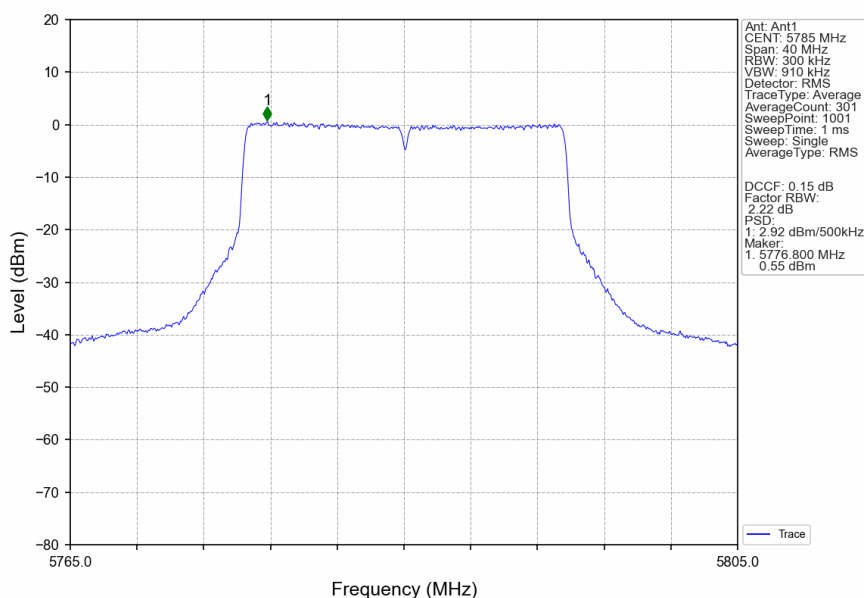
802.11ax(HEW20)_MCH_5785MHz_RU242_Left_Ant1_NTNV
