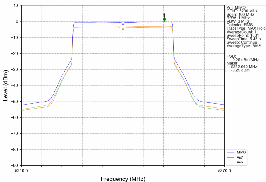
802.11ax(HEW80)_MCH_5290MHz_RU996_Left_MIMO_NTNV
