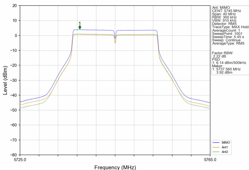
802.11n(HT20)_LCH_5745MHz_MIMO_NTNV
