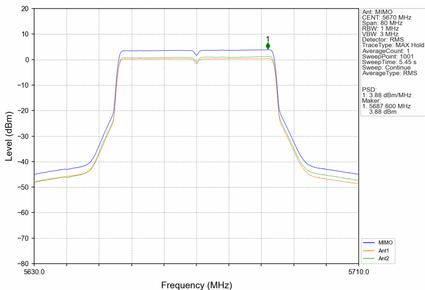
802.11ax(HEW40)_HCH_5670MHz_RU484_Left_MIMO_NTNV
