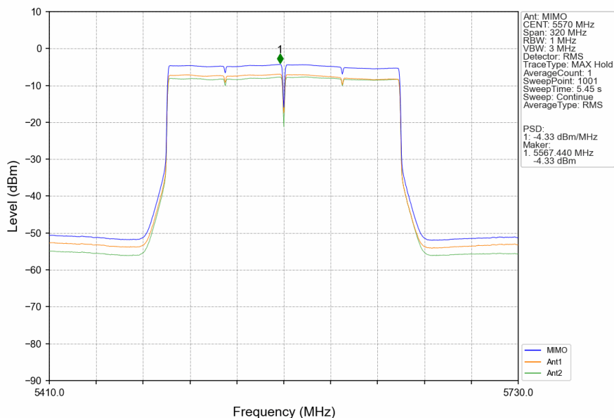
802.11ax(HEW160)_MCH_5570MHz_2xRU996_Left_MIMO_NTNV
