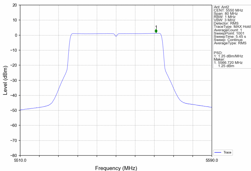
802.11ax(HEW40)_MCH_5550MHz_RU484_Left_Ant2_NTNV
