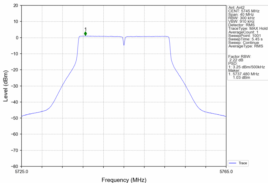
802.11n(HT20)_LCH_5745MHz_Ant2_NTNV
