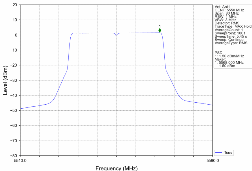
802.11ax(HEW40)_MCH_5550MHz_RU484_Left_Ant1_NTNV
