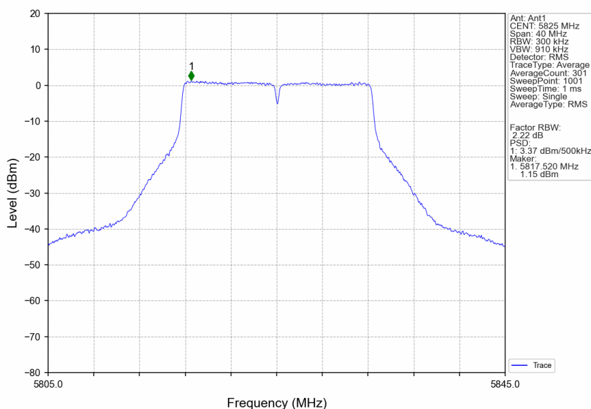
802.11a_HCH_5825MHz_Ant1_NTNV
