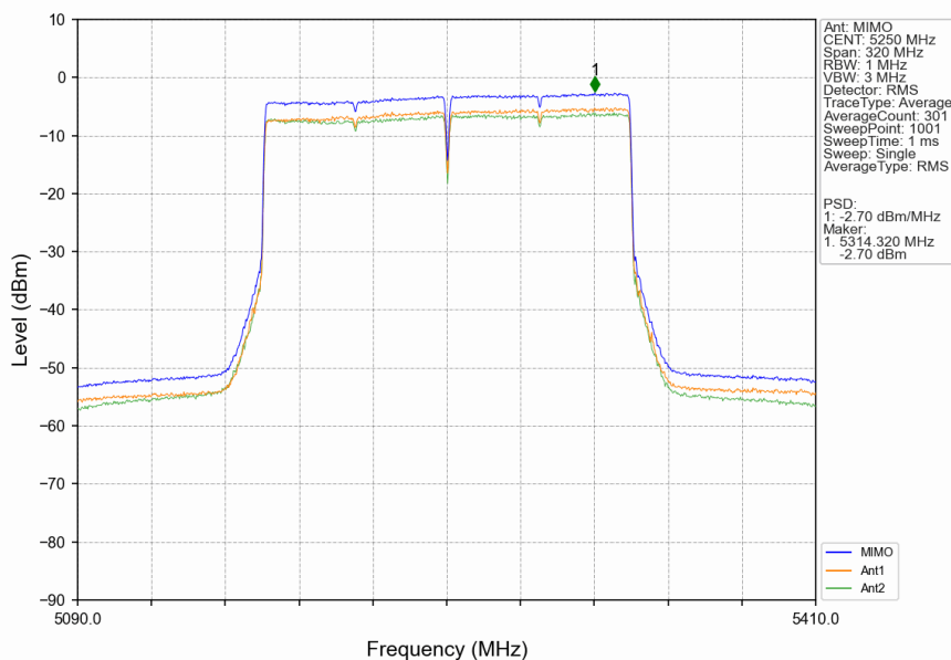
802.11ax(HEW160)_MCH_5250MHz_2xRU996_Left_MIMO_NTNV
