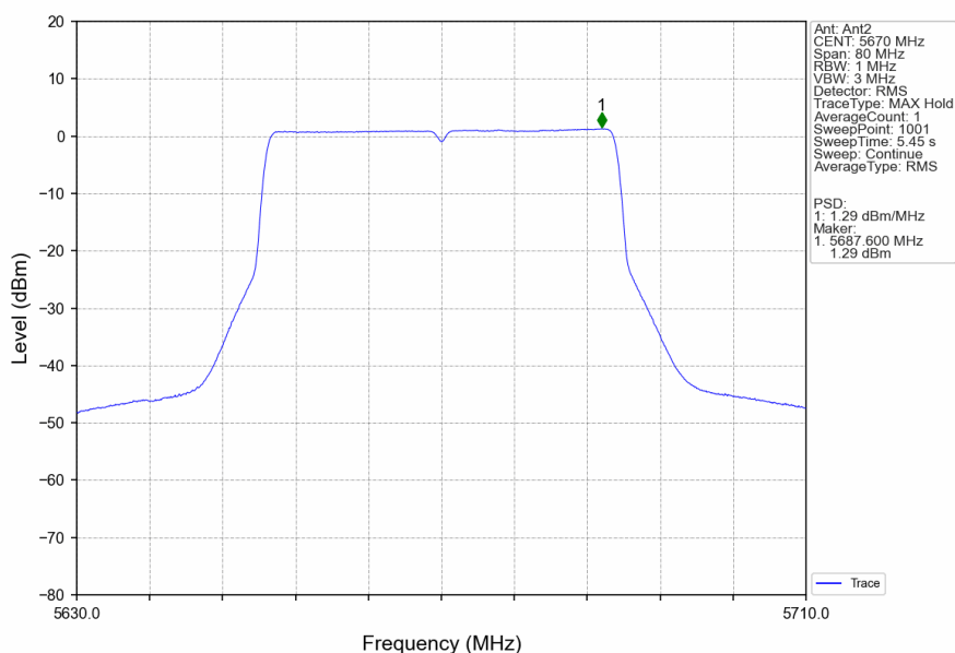
802.11ax(HEW40)_HCH_5670MHz_RU484_Left_Ant2_NTNV
