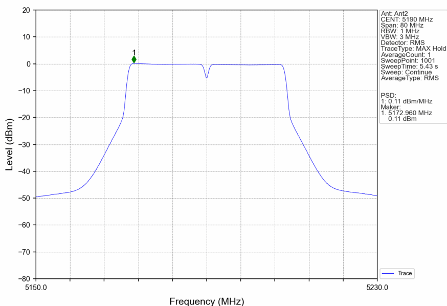
802.11ac(VHT40)_LCH_5190MHz_Ant2_NTNV
