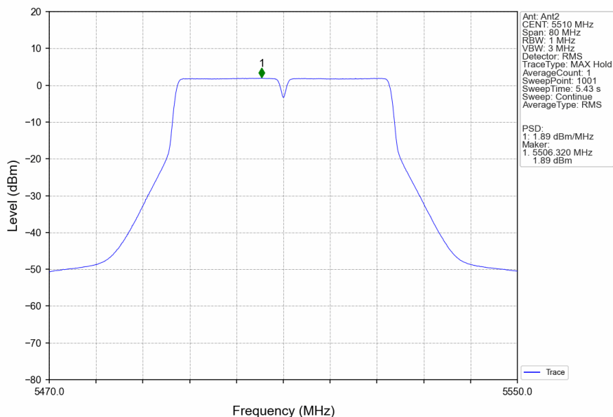
802.11ac(VHT40)_LCH_5510MHz_Ant2_NTNV
