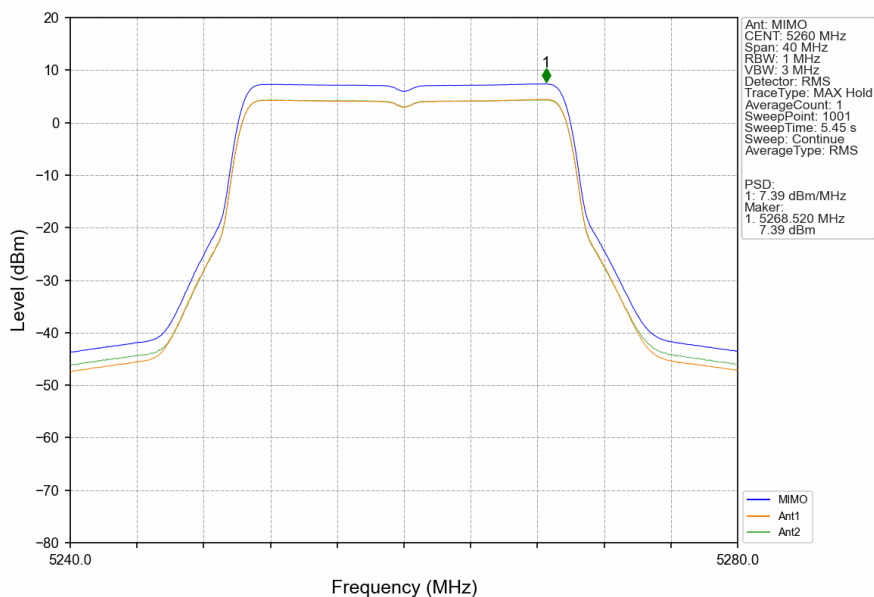
802.11ax(HEW20)_LCH_5260MHz_RU242_Left_MIMO_NTNV
