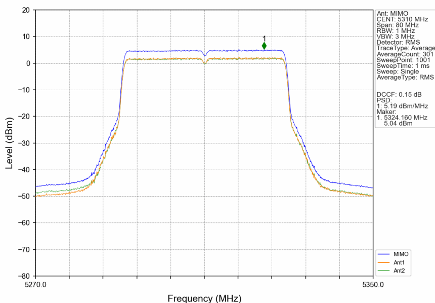
802.11ax(HEW40)_HCH_5310MHz_RU484_Left_MIMO_NTNV
