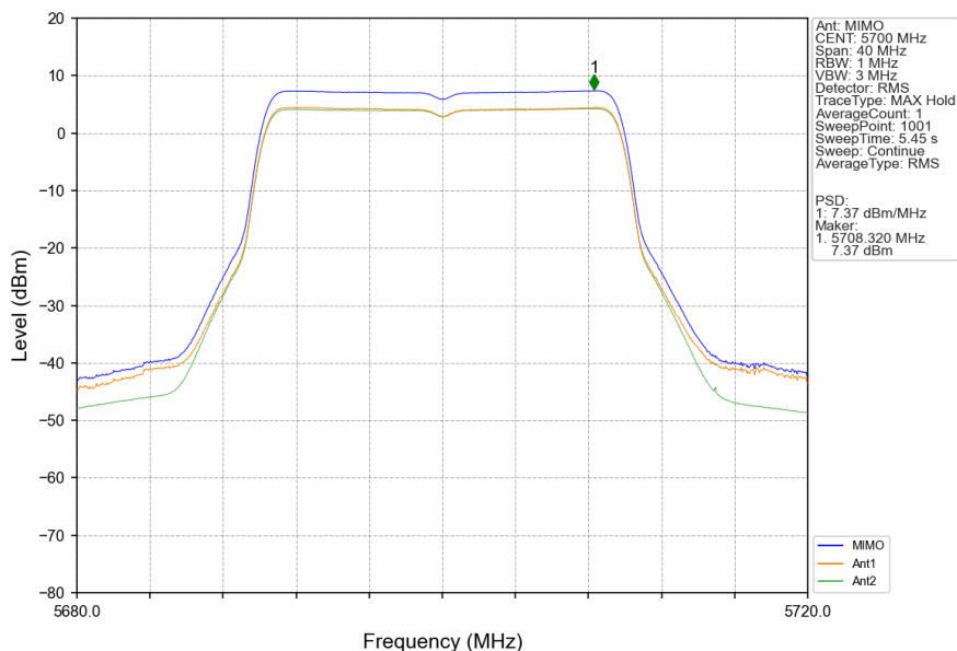
802.11ax(HEW20)_HCH_5700MHz_RU242_Left_MIMO_NTNV
