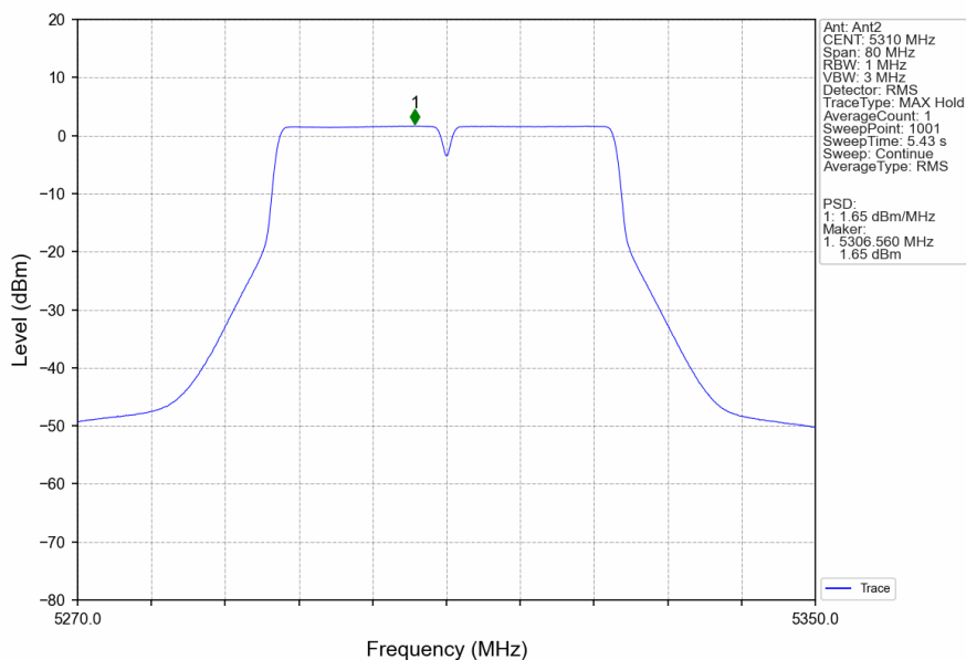
802.11ac(VHT40)_HCH_5310MHz_Ant2_NTNV
