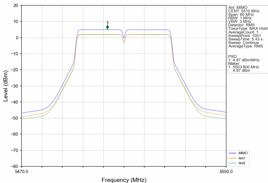
802.11ac(VHT40)_LCH_5510MHz_MIMO_NTNV
