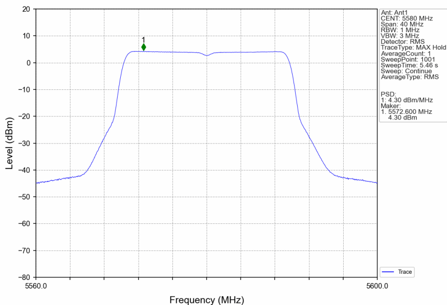
802.11ax(HEW20)_MCH_5580MHz_RU242_Left_Ant1_NTNV
