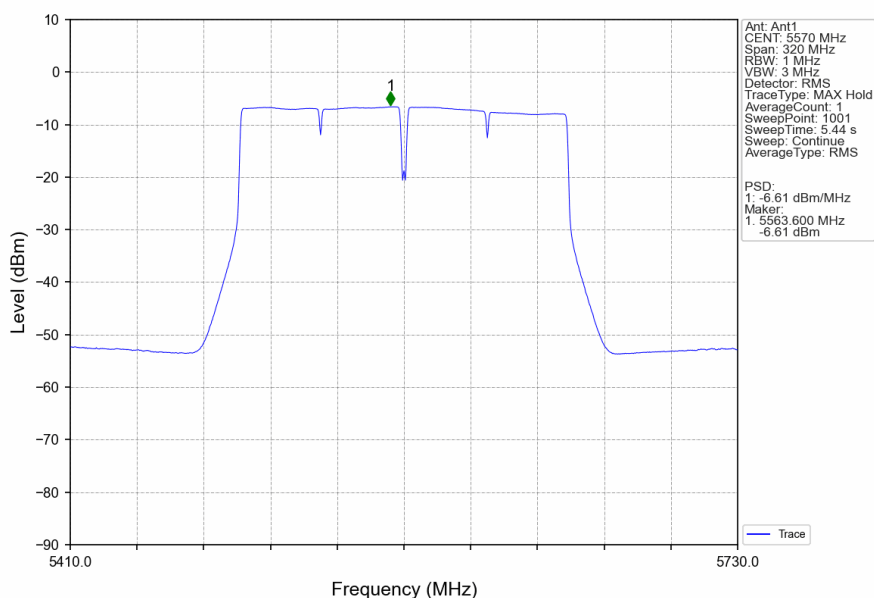
802.11ac(VHT160)_MCH_5570MHz_Ant1_NTNV
