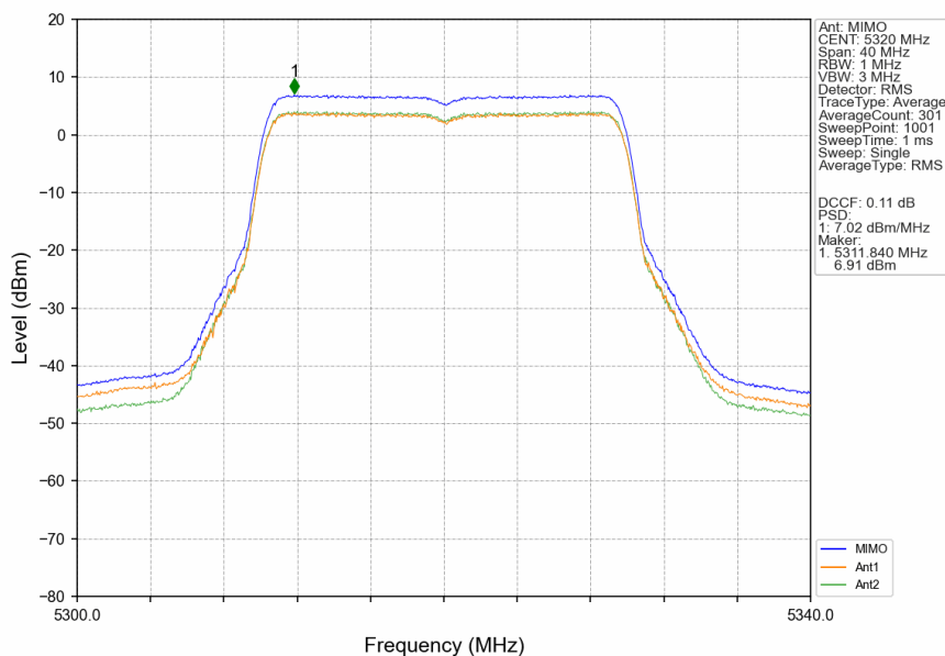
802.11ax(HEW20)_HCH_5320MHz_RU242_Left_MIMO_NTNV
