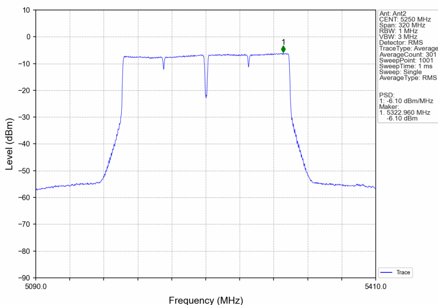
802.11ac(VHT160)_MCH_5250MHz_Ant2_NTNV
