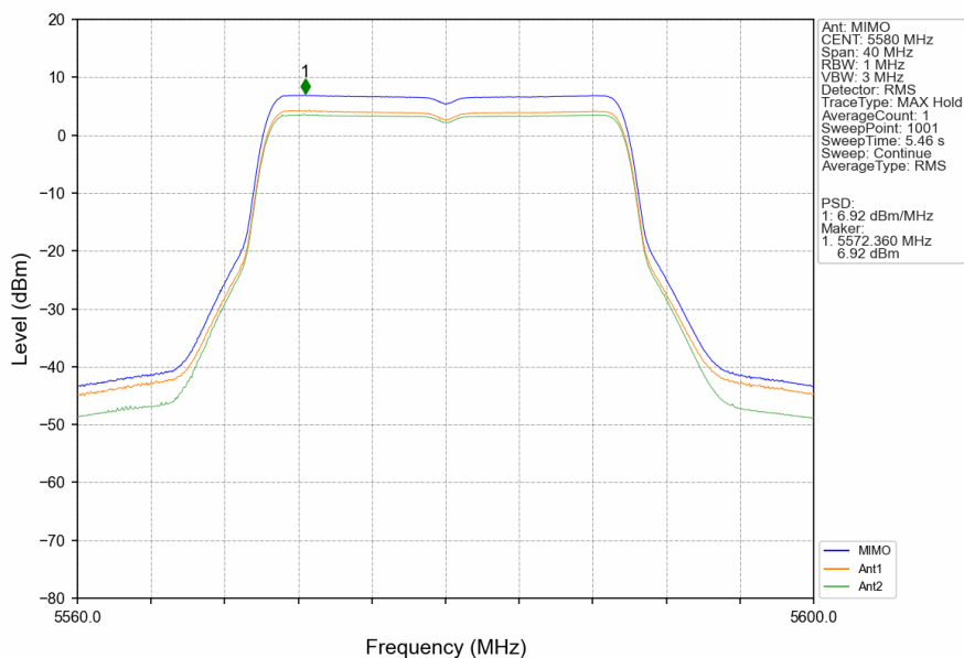
802.11ax(HEW20)_MCH_5580MHz_RU242_Left_MIMO_NTNV
