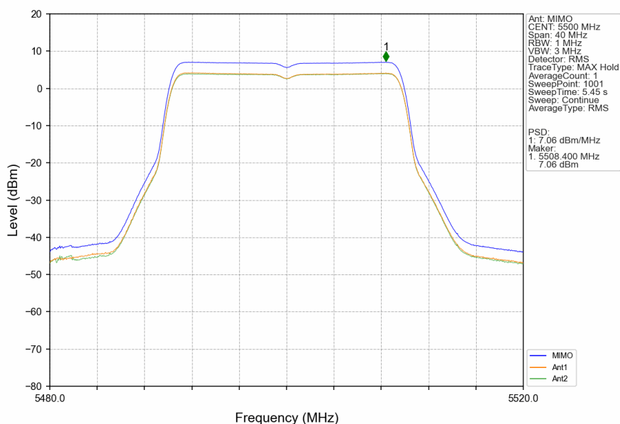
802.11ax(HEW20)_LCH_5500MHz_RU242_Left_MIMO_NTNV
