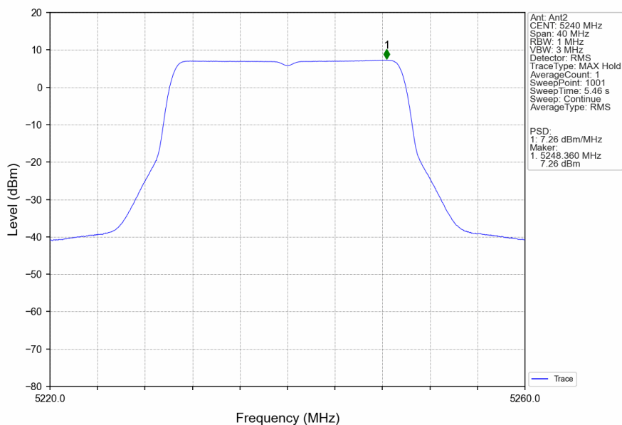
802.11ax(HEW20)_HCH_5240MHz_RU242_Left_Ant2_NTNV
