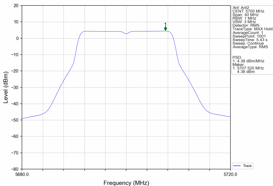
802.11ac(VHT20)_HCH_5700MHz_Ant2_NTNV
