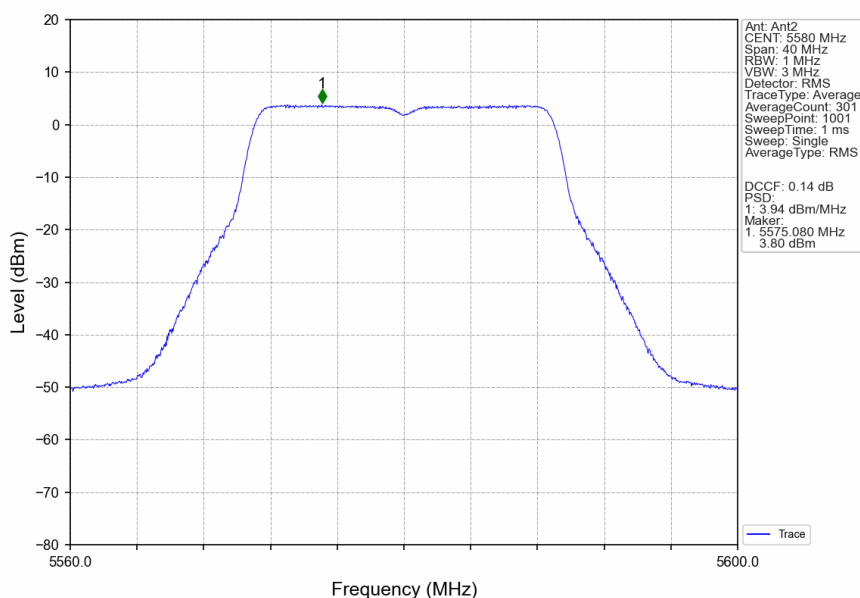
802.11ac(VHT20)_MCH_5580MHz_Ant2_NTNV
