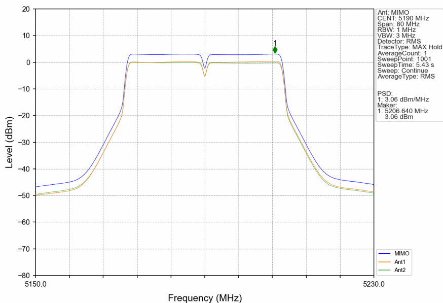
802.11ac(VHT40)_LCH_5190MHz_MIMO_NTNV
