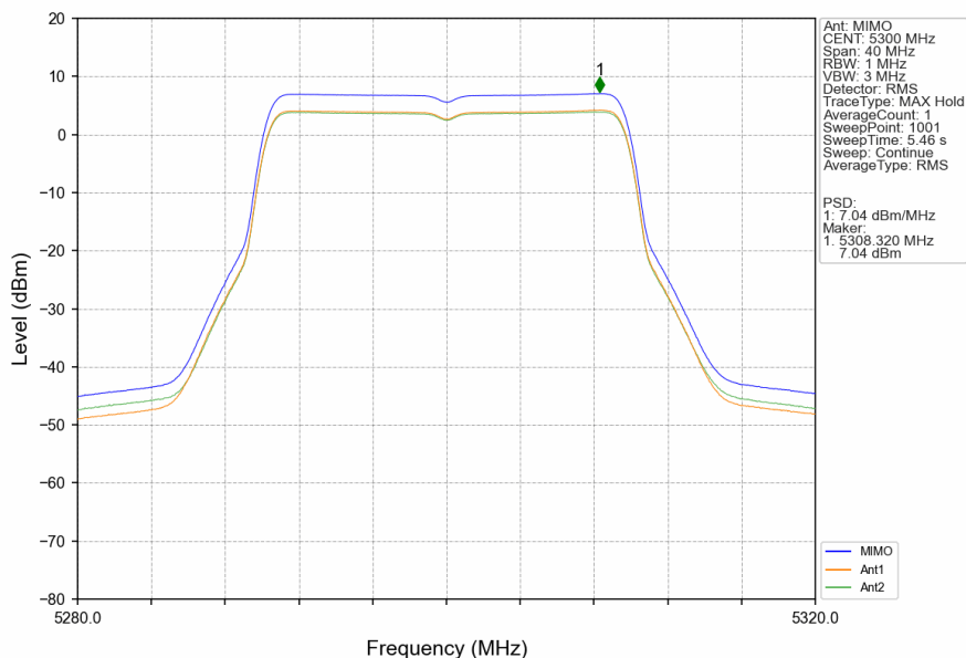
802.11ax(HEW20)_MCH_5300MHz_RU242_Left_MIMO_NTNV
