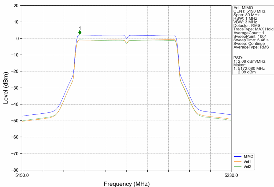
802.11ax(HEW40)_LCH_5190MHz_RU484_Left_MIMO_NTNV
