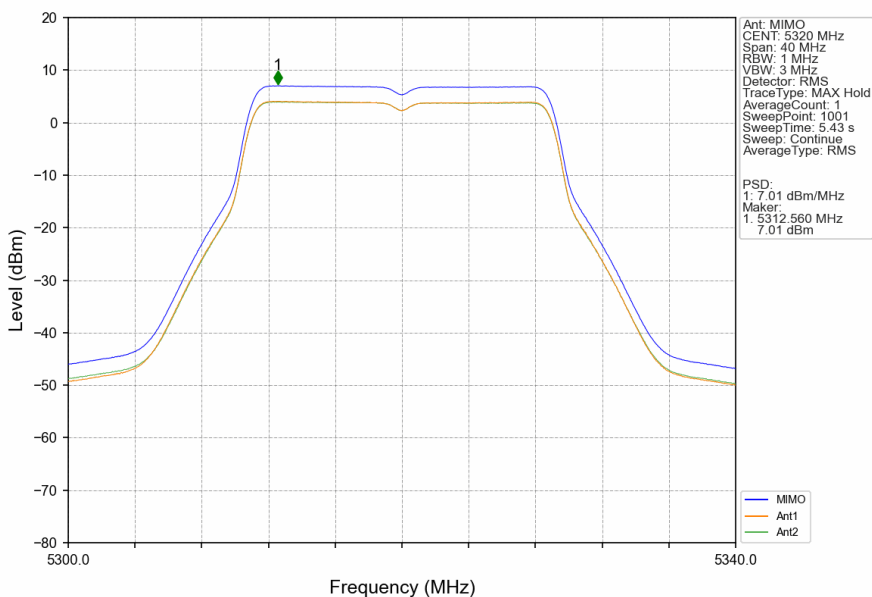
802.11ac(VHT20)_HCH_5320MHz_MIMO_NTNV
