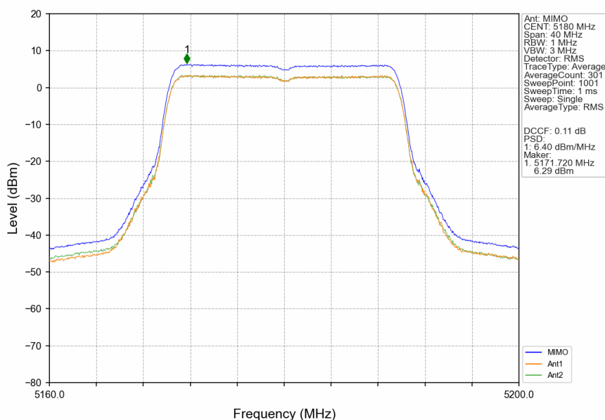
802.11ax(HEW20)_LCH_5180MHz_RU242_Left_MIMO_NTNV
