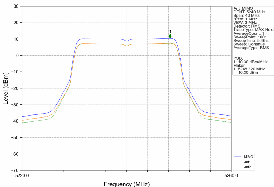
802.11ax(HEW20)_HCH_5240MHz_RU242_Left_MIMO_NTNV
