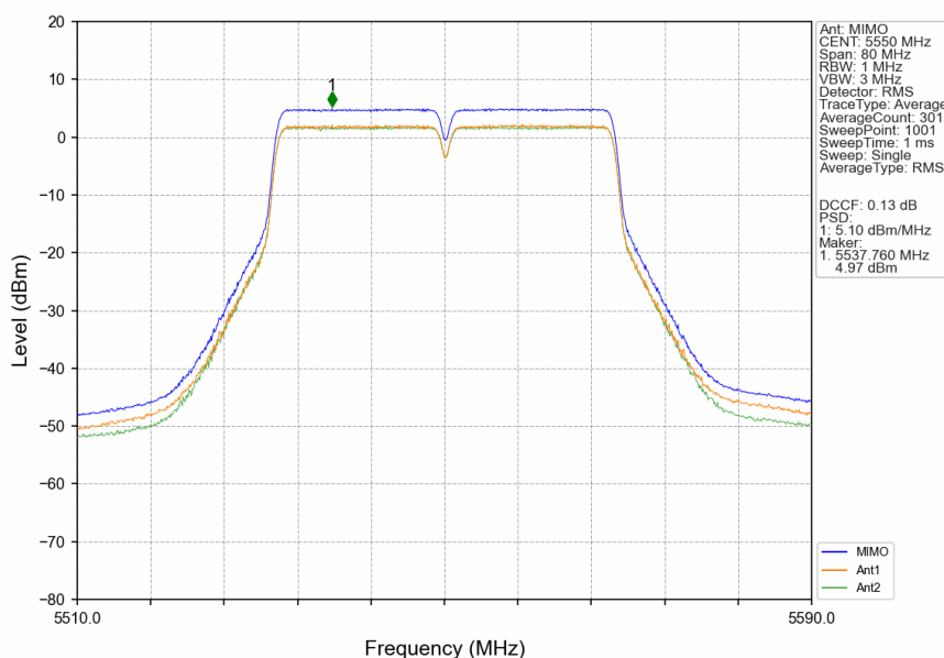
802.11ac(VHT40)_MCH_5550MHz_MIMO_NTNV
