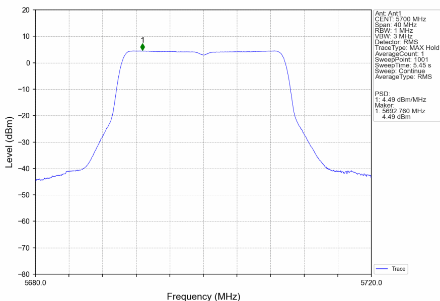
802.11ax(HEW20)_HCH_5700MHz_RU242_Left_Ant1_NTNV
