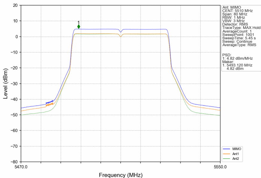
802.11ax(HEW40)_LCH_5510MHz_RU484_Left_MIMO_NTNV
