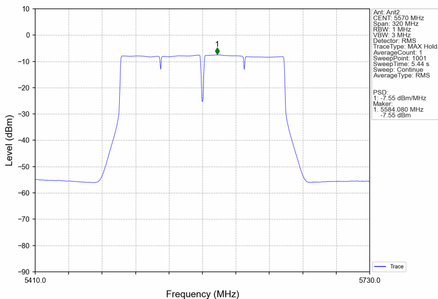
802.11ac(VHT160)_MCH_5570MHz_Ant2_NTNV
