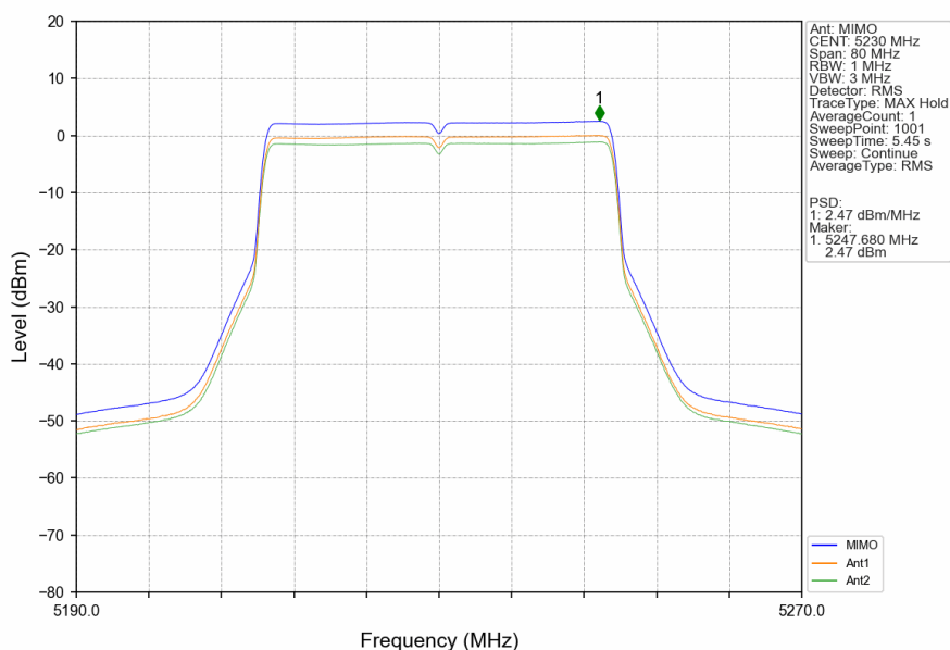
802.11ax(HEW40)_HCH_5230MHz_RU484_Left_MIMO_NTNV
