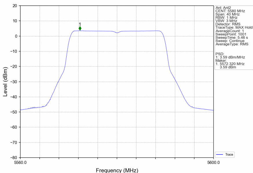
802.11ax(HEW20)_MCH_5580MHz_RU242_Left_Ant2_NTNV
