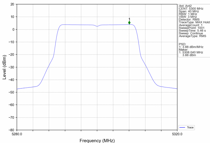
802.11ax(HEW20)_MCH_5300MHz_RU242_Left_Ant2_NTNV
