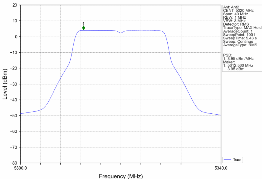
802.11ac(VHT20)_HCH_5320MHz_Ant2_NTNV
