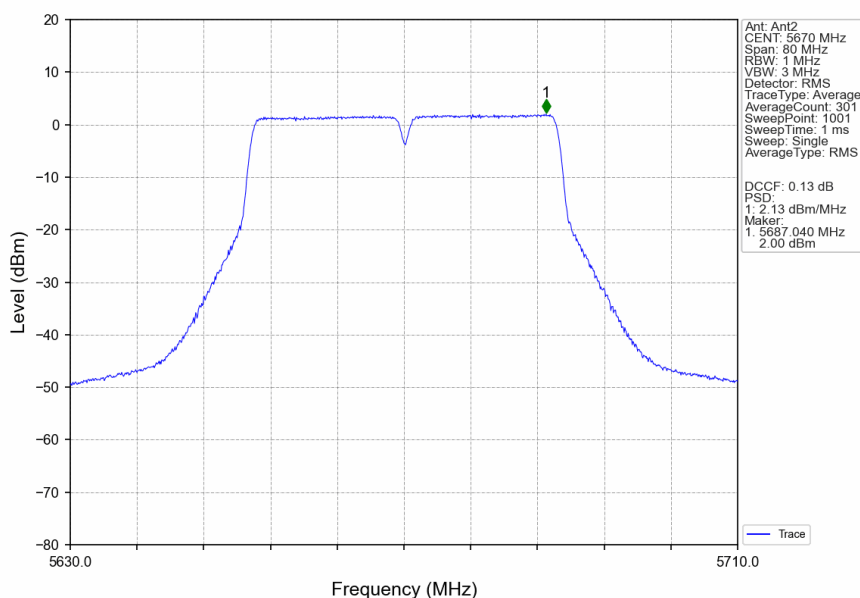
802.11ac(VHT40)_HCH_5670MHz_Ant2_NTNV
