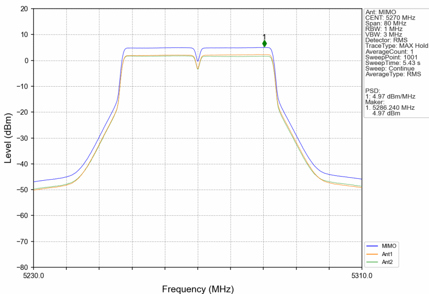
802.11ac(VHT40)_LCH_5270MHz_MIMO_NTNV
