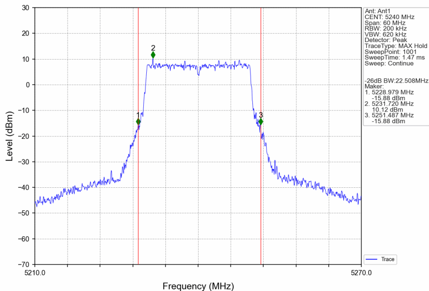
802.11ax(HEW20)_HCH_5240MHz_RU242_Left_Ant1_NTNV
