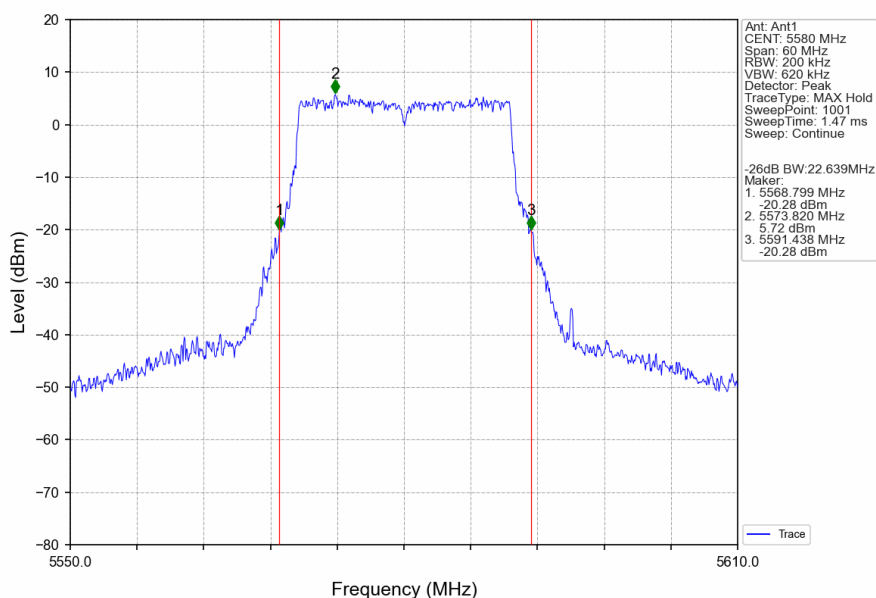
802.11ax(HEW20)_MCH_5580MHz_RU242_Left_Ant1_NTNV
