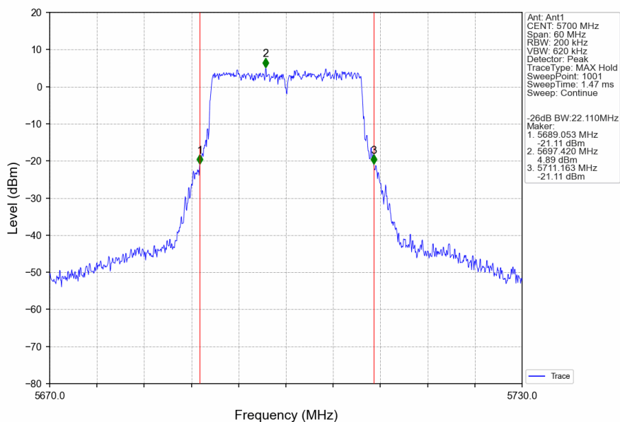
802.11ax(HEW20)_HCH_5700MHz_RU242_Left_Ant1_NTNV
