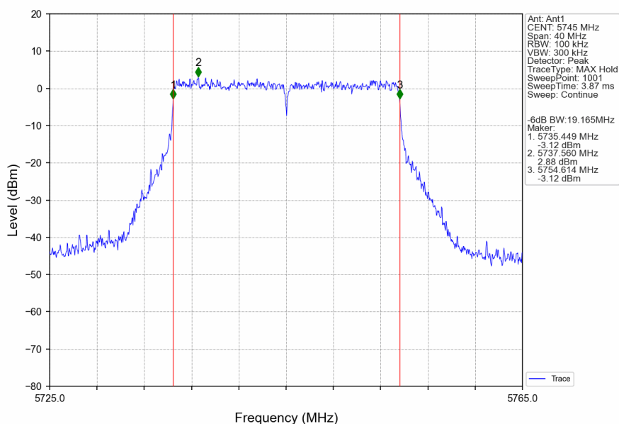
802.11ax(HEW20)_LCH_5745MHz_RU242_Left_Ant1_NTNV
