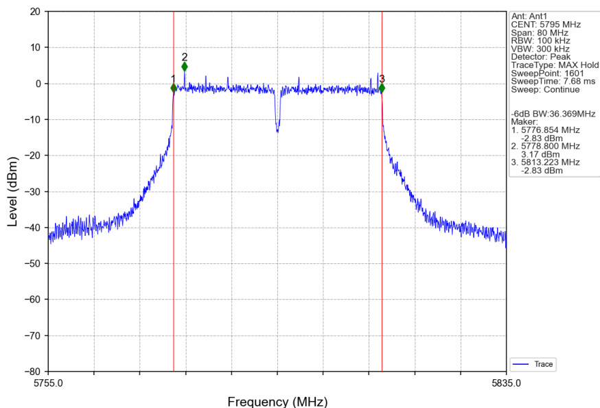
802.11ac(VHT40)_HCH_5795MHz_Ant1_NTNV
