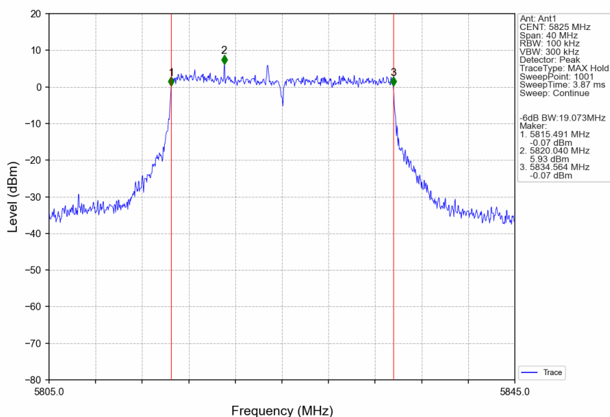
802.11ax(HEW20)_HCH_5825MHz_RU242_Left_Ant1_NTNV
