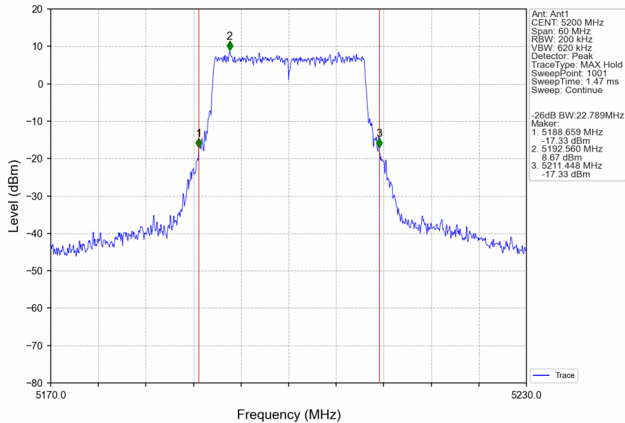
802.11ax(HEW20)_MCH_5200MHz_RU242_Left_Ant1_NTNV
