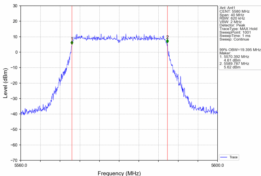
802.11ax(HEW20)_MCH_5580MHz_RU242_Left_Ant1_NTNV
