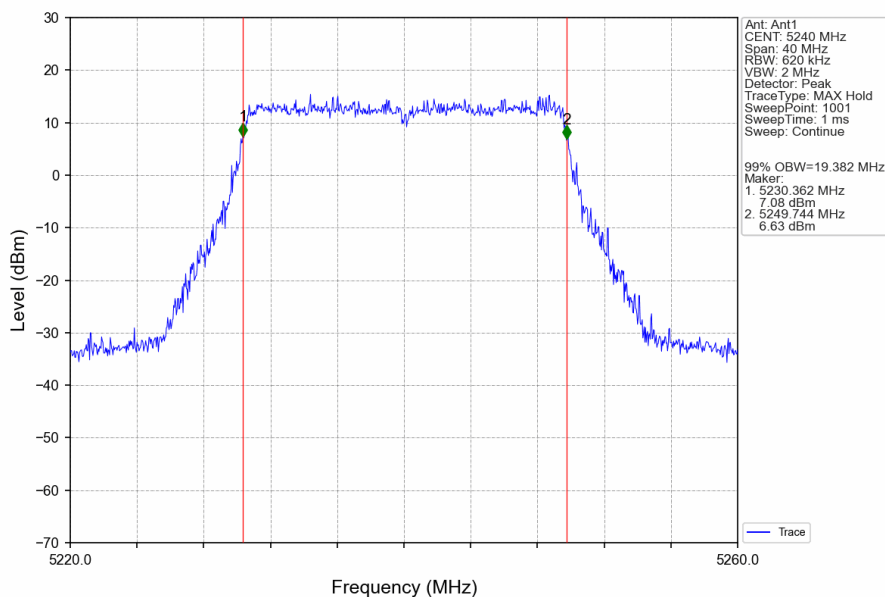
802.11ax(HEW20)_HCH_5240MHz_RU242_Left_Ant1_NTNV
