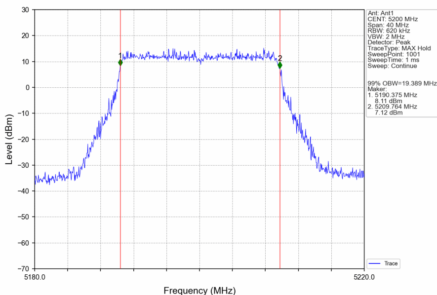
802.11ax(HEW20)_MCH_5200MHz_RU242_Left_Ant1_NTNV
