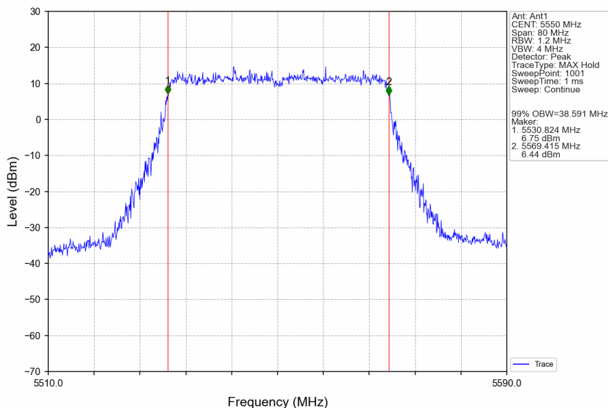
802.11ax(HEW40)_MCH_5550MHz_RU484_Left_Ant1_NTNV
