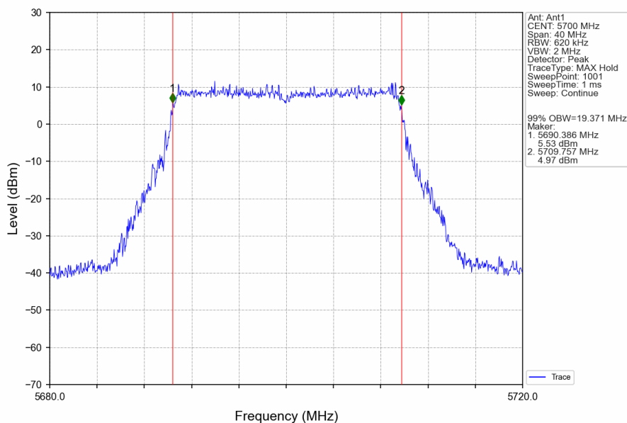
802.11ax(HEW20)_HCH_5700MHz_RU242_Left_Ant1_NTNV
