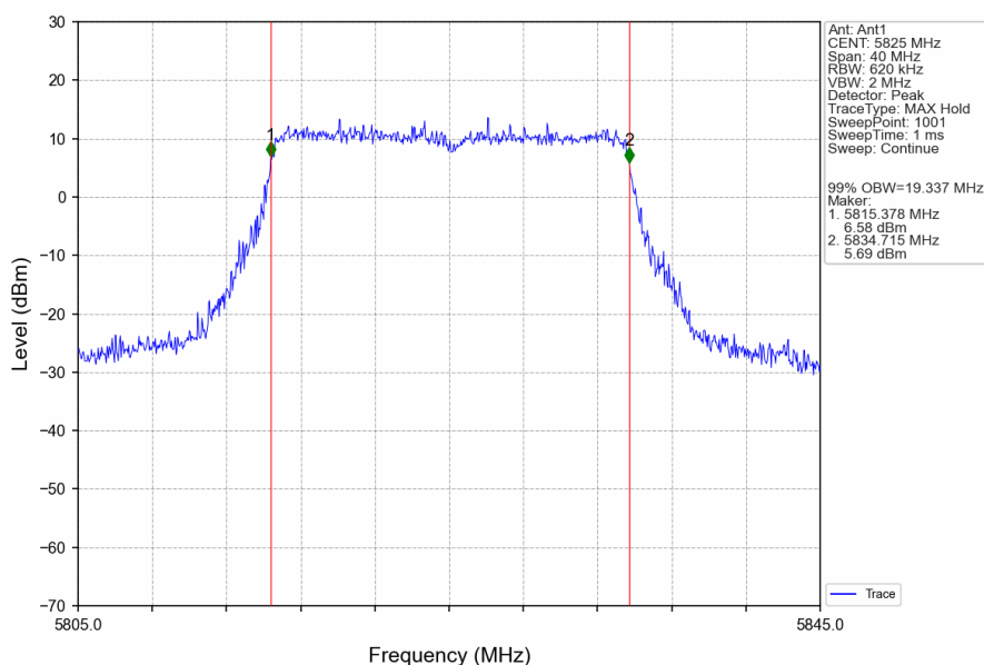
802.11ax(HEW20)_HCH_5825MHz_RU242_Left_Ant1_NTNV
