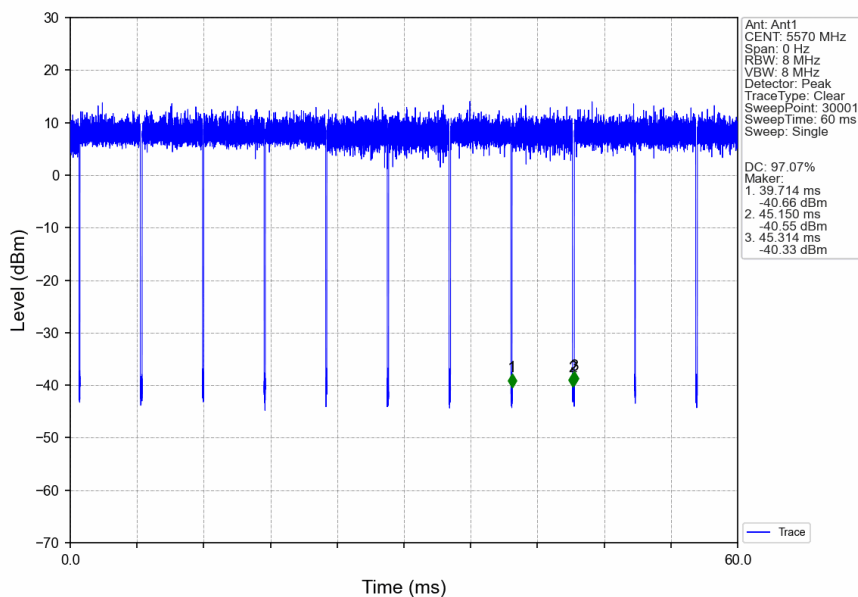
802.11ac(VHT160)_MCH_5570MHz_Ant1_NTNV
