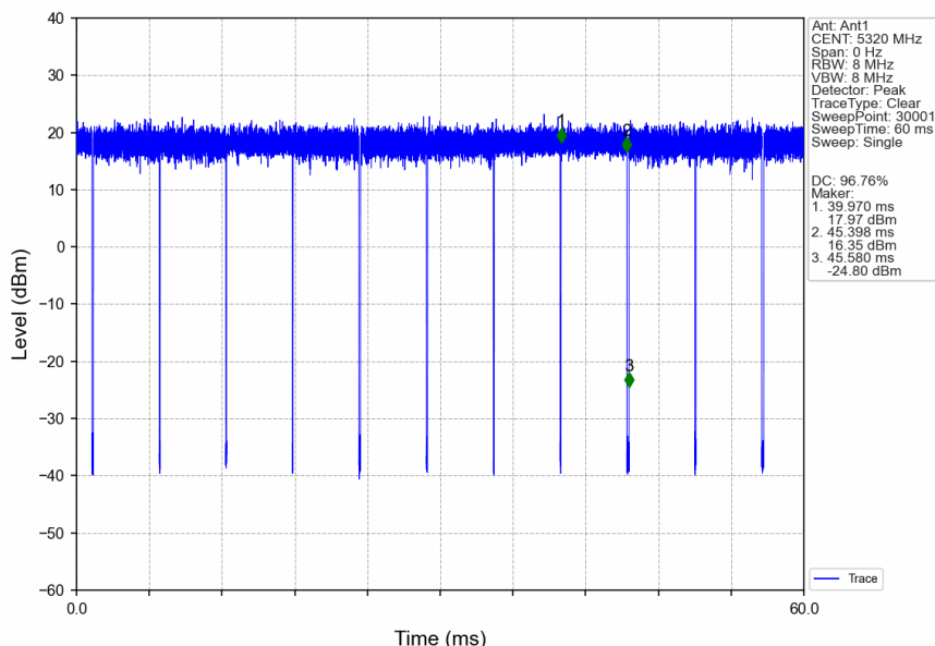
802.11ac(VHT20)_HCH_5320MHz_Ant1_NTNV
