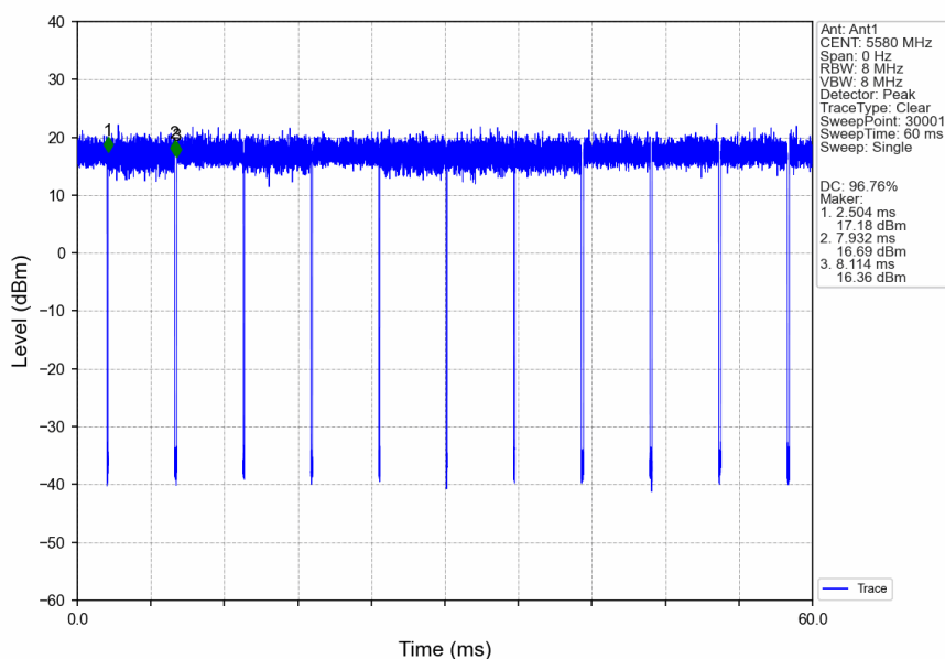
802.11ac(VHT20)_MCH_5580MHz_Ant1_NTNV
