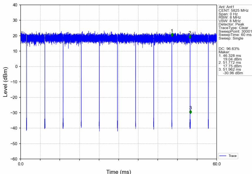
802.11ax(HEW20)_HCH_5825MHz_RU242_Left_Ant1_NTNV
