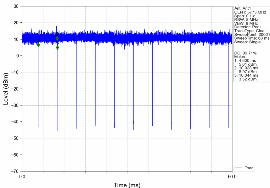
802.11ac(VHT80)_MCH_5775MHz_Ant1_NTNV
