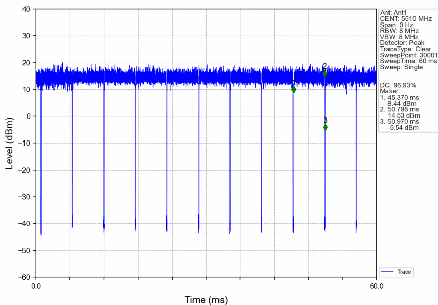
802.11ac(VHT40)_LCH_5510MHz_Ant1_NTNV
