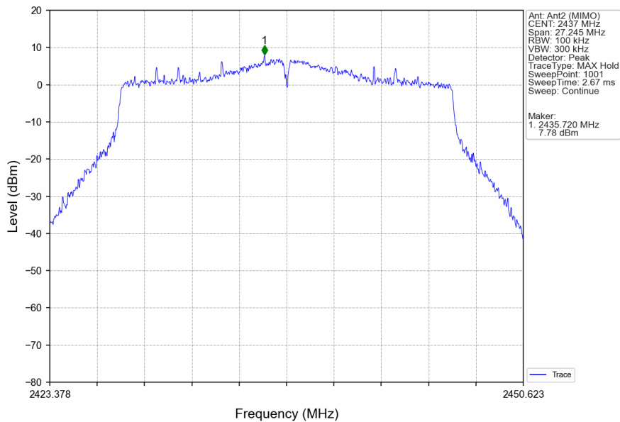
802.11ax(HEW20)_MCH_2437MHz_SU_/_Ant2 (MIMO)_NTNV
