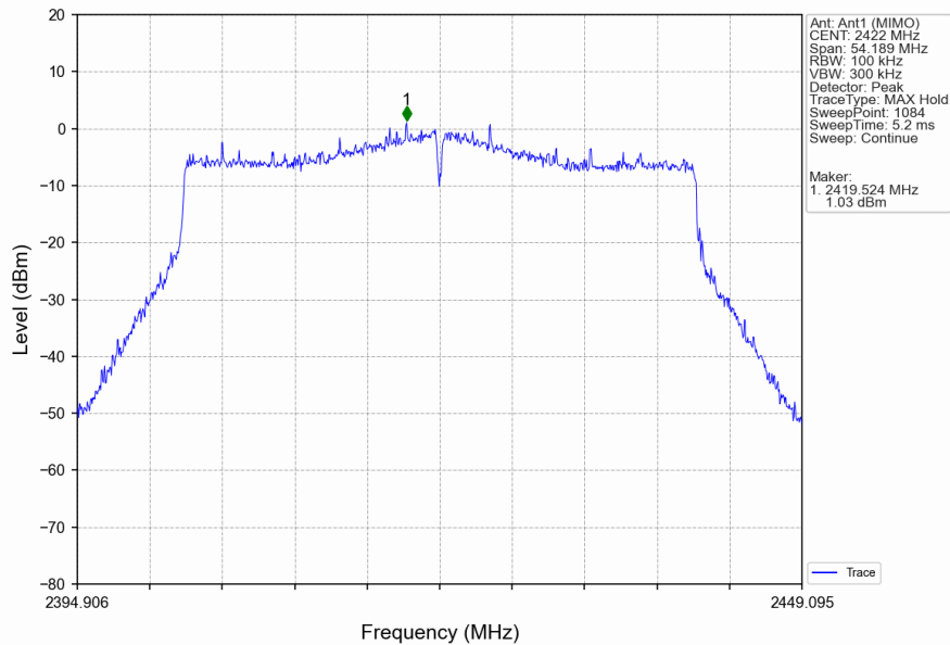
802.11ax(HEW40)_LCH_2422MHz_SU_/_Ant1 (MIMO)_NTNV
