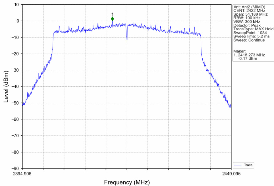
802.11ax(HEW40)_LCH_2422MHz_SU_/_Ant2 (MIMO)_NTNV
