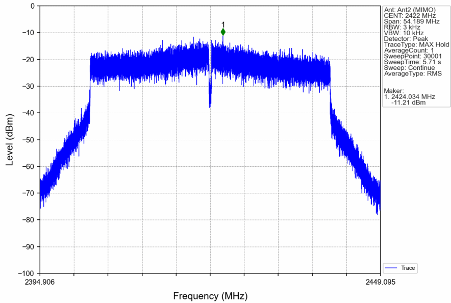
802.11ax(HEW40)_LCH_2422MHz_SU_/_Ant2 (MIMO)_NTNV
