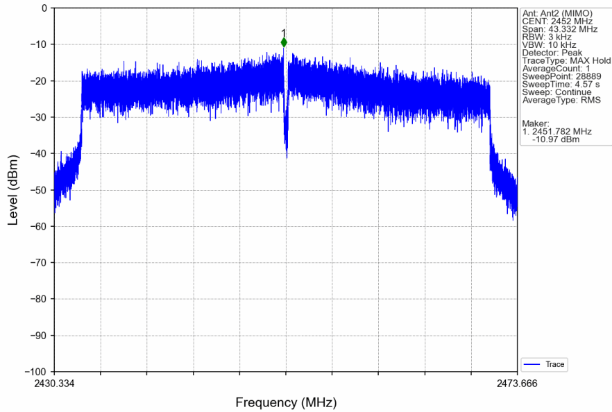
802.11ax(HEW40)_HCH_2452MHz_SU_/_Ant2 (MIMO)_NTNV
