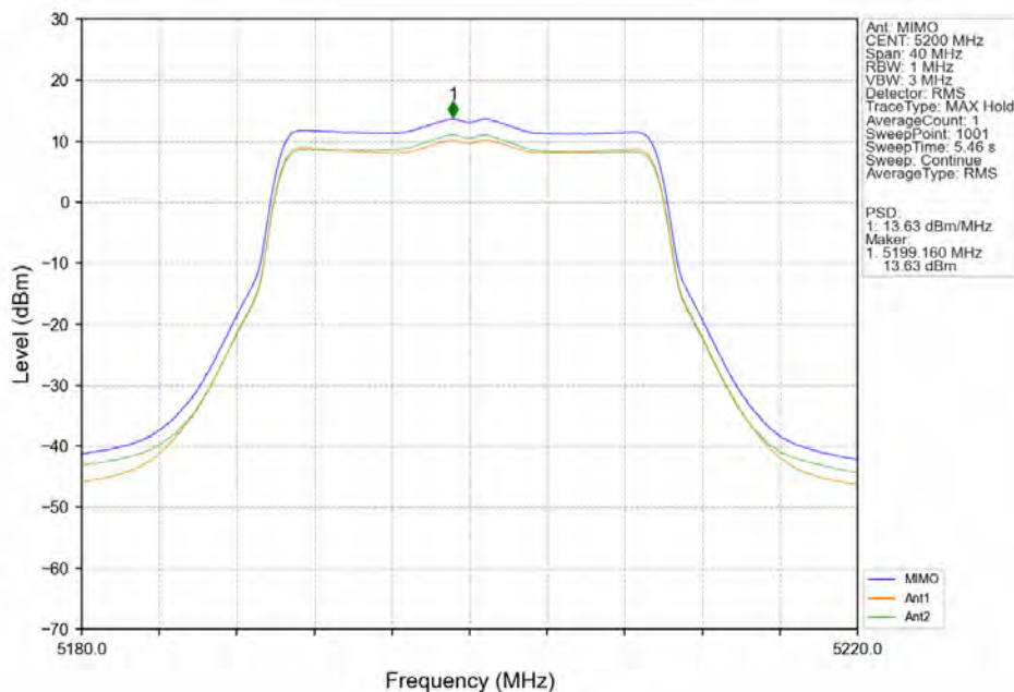
802.11be(EHT20)_MCH_5200MHz_SU_/_MIMO_NTNV
