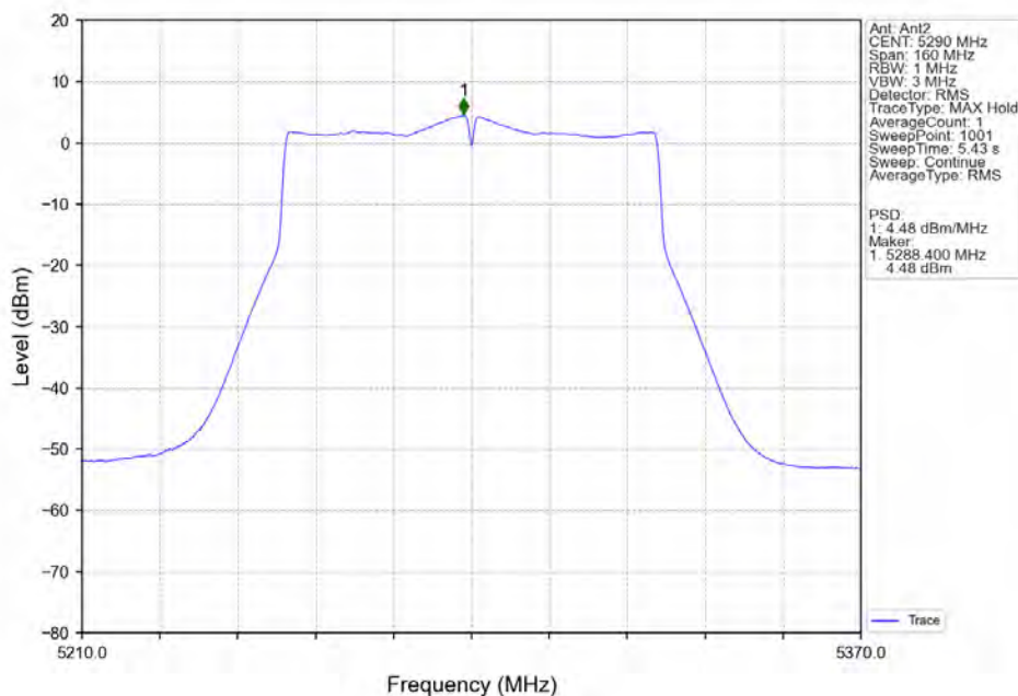
802.11ac(VHT80)_MCH_5290MHz_MIMO_NTNV
