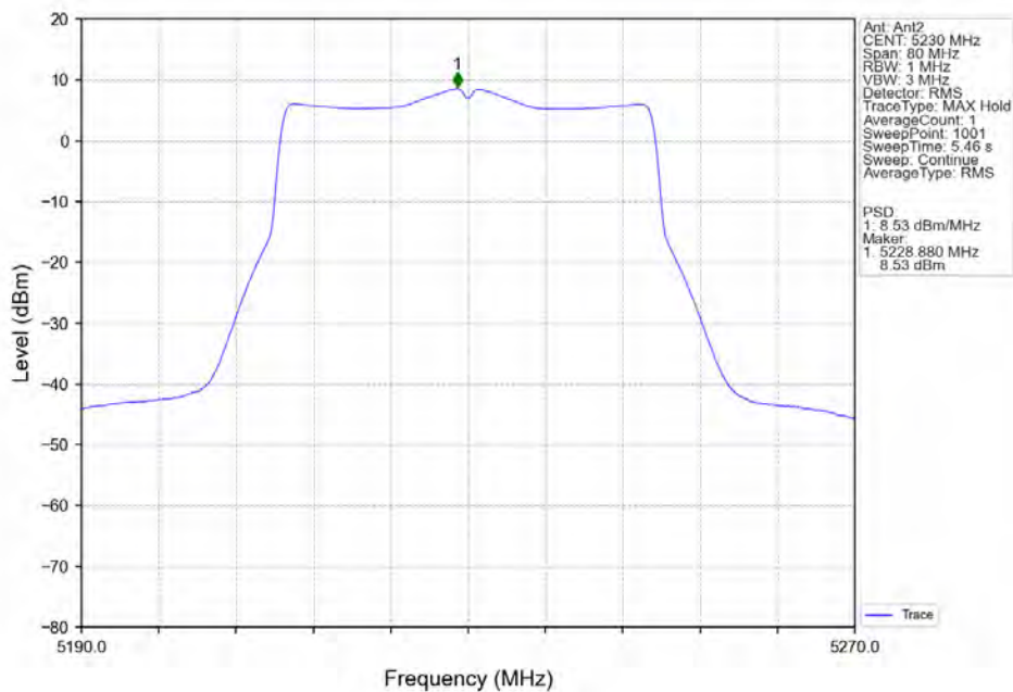
802.11ax(HEW40)_HCH_5230MHz_SU_/_Ant2_NTNV
