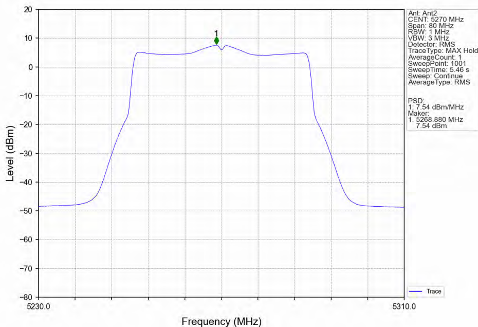
802.11ax(HEW40)_LCH_5270MHz_SU_ / _MIMO_NTNV
