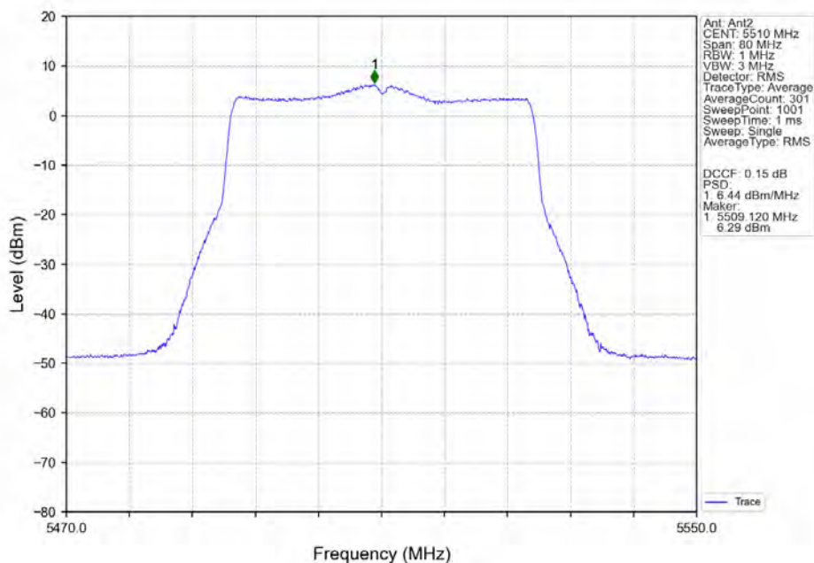
802.11ax(HEW40)_LCH_5510MHz_SU_ / _MIMO_NTNV
