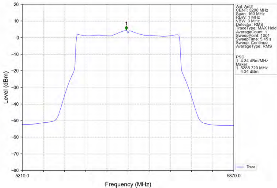
802.11ax(HEW80)_MCH_5290MHz_SU_/_MIMO_NTNV
