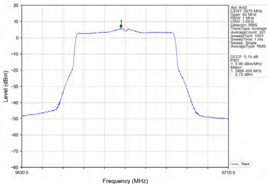
802.11be(EHT40)_HCH_5670MHz_SU_/_MIMO_NTNV
