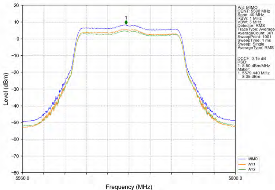
802.11ax(HEW20)_MCH_5580MHz_SU_/_MIMO_NTNV
