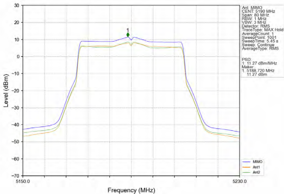
802.11ax(HEW40)_LCH_5190MHz_SU_ / _MIMO_NTNV
