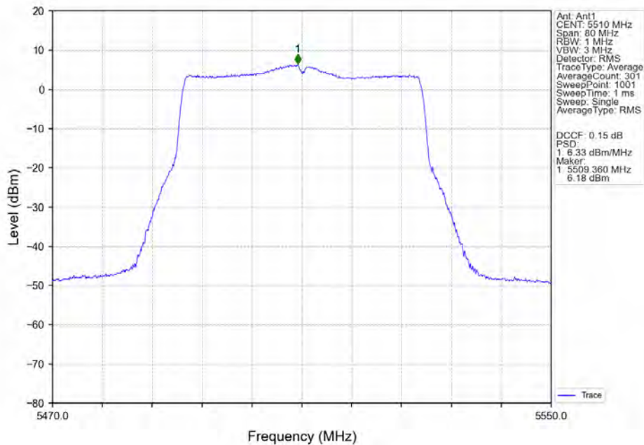
802.11ax(HEW40)_LCH_5510MHz_SU_/_Ant1_NTNV
