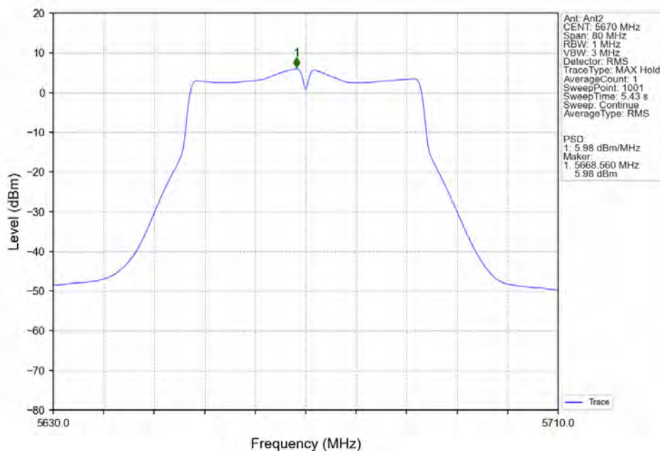
802.11ac(VHT40)_HCH_5670MHz_MIMO_NTNV
