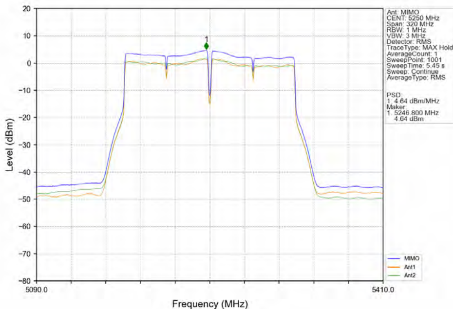
802.11ac(VHT160)_MCH_5250MHz_MIMO_NTNV
