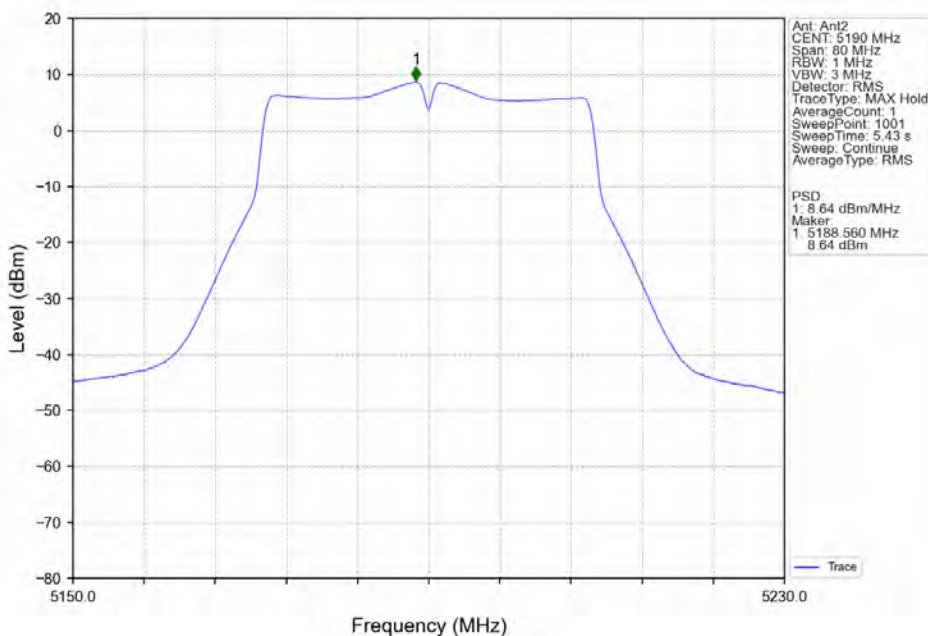
802.11n(HT40)_LCH_5190MHz_MIMO_NTNV
