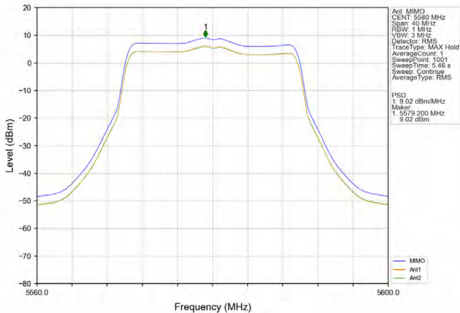
802.11be(EHT20)_MCH_5580MHz_SU_/_MIMO_NTNV
