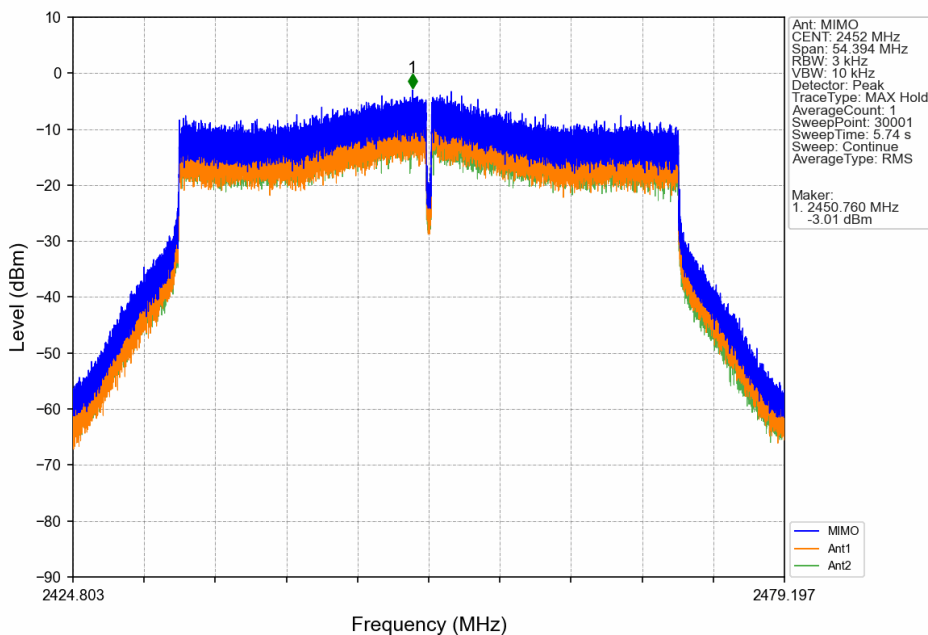
802.11ax(HEW40)_HCH_2452MHz_SU_/_MIMO_NTNV
