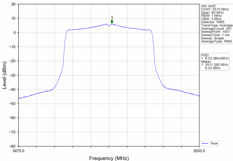
802.11ax(HEW40)_LCH_5510MHz_RU484_Left_MIMO_NTNV
