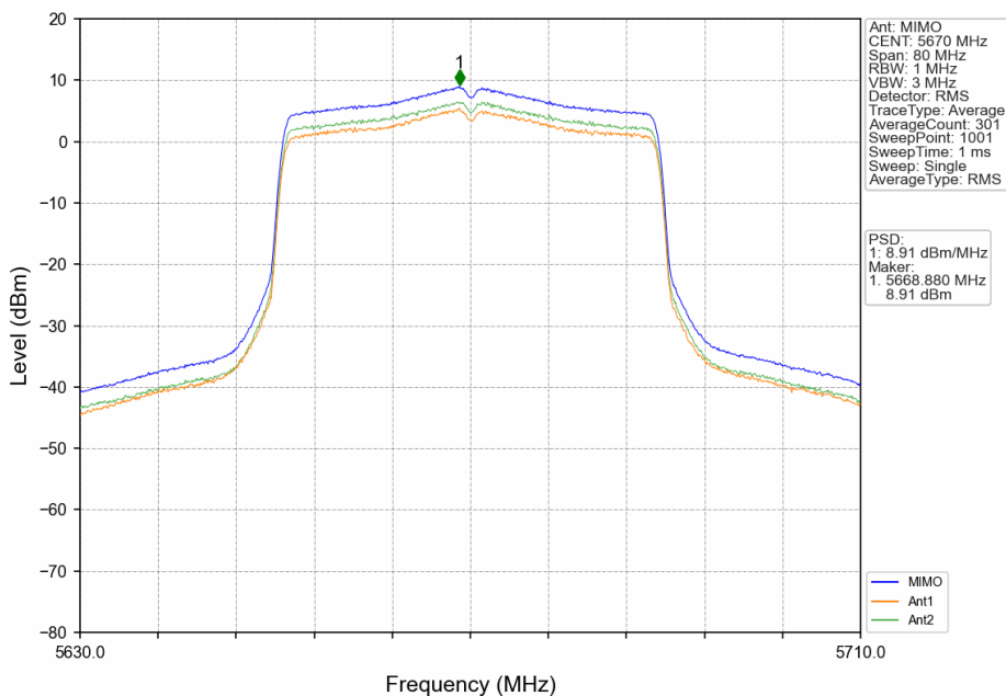
802.11ax(HEW40)_HCH_5670MHz_RU484_Left_MIMO_NTNV
