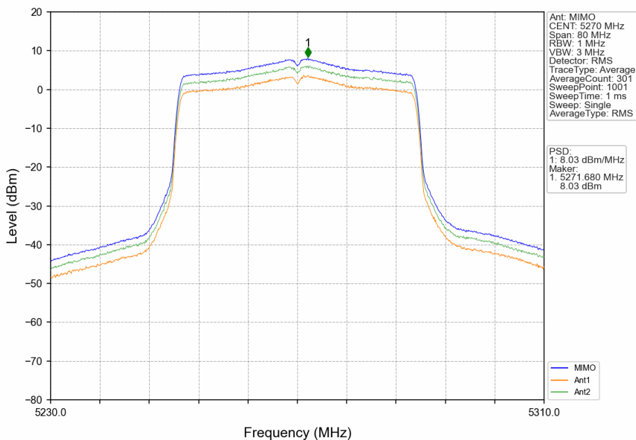
802.11ax(HEW40)_LCH_5270MHz_RU484_Left_MIMO_NTNV
