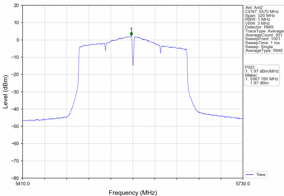
802.11ac(VHT160)_MCH_5570MHz_Ant2_NTNV
