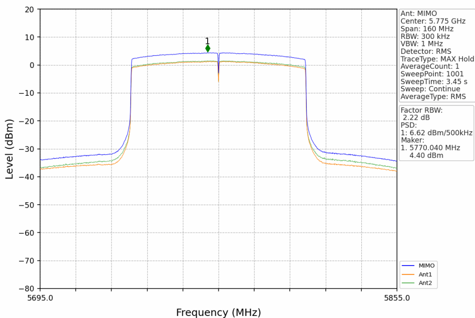
802.11ax(HEW80)_MCH_5775MHz_RU996_Left_MIMO_NTNV
