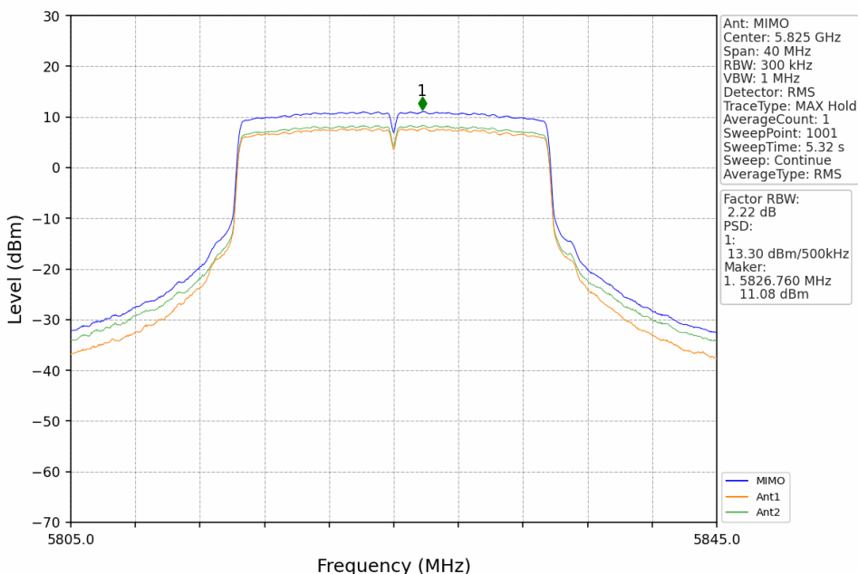
802.11ax(HEW20)_HCH_5825MHz_RU242_Left_MIMO_NTNV
