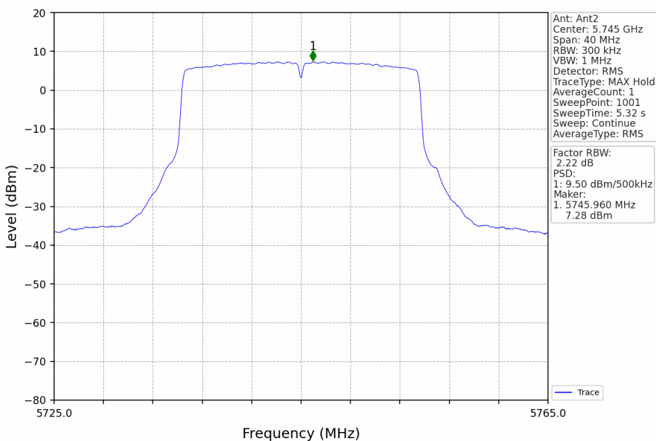
802.11ax(HEW20)_LCH_5745MHz_RU242_Left_MIMO_NTNV
