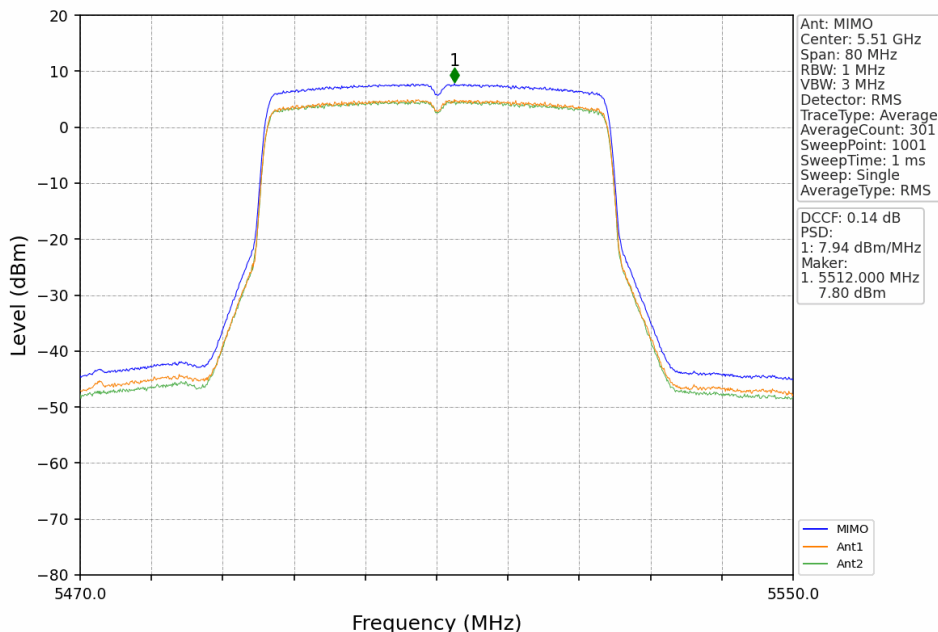
802.11ax(HEW40)_LCH_5510MHz_RU484_Left_MIMO_NTNV
