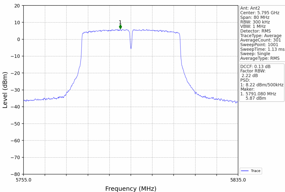
802.11ac(VHT40)_HCH_5795MHz_MIMO_NTNV
