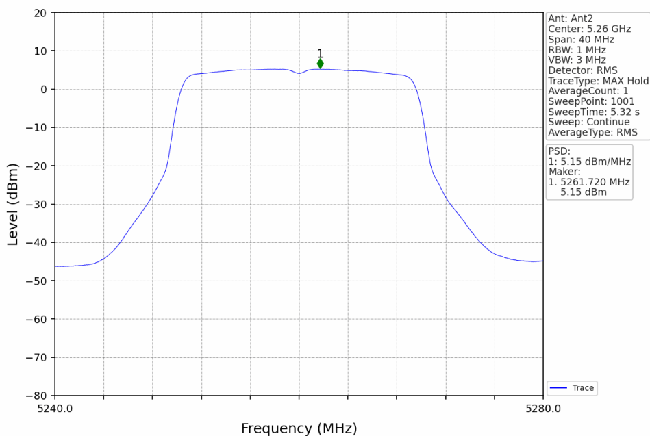
802.11ax(HEW20)_LCH_5260MHz_RU242_Left_MIMO_NTNV
