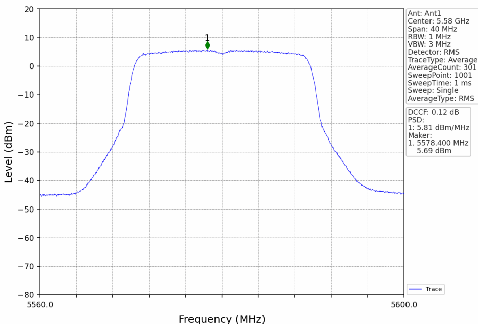
802.11ax(HEW20)_MCH_5580MHz_RU242_Left_Ant1_NTNV
