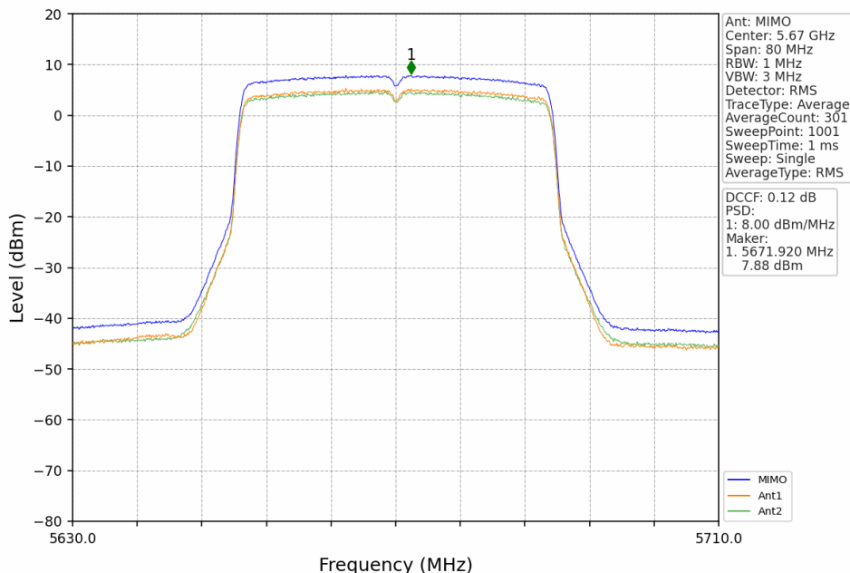
802.11ax(HEW40)_HCH_5670MHz_RU484_Left_MIMO_NTNV
