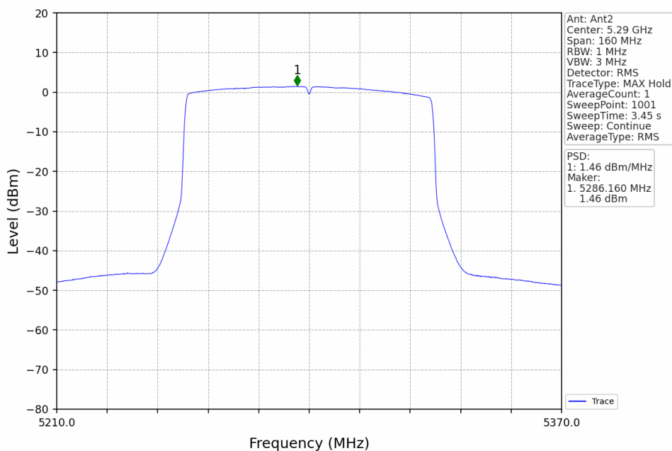
802.11ax(HEW80)_MCH_5290MHz_RU996_Left_MIMO_NTNV
