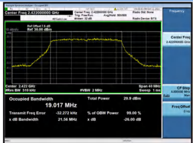
802.11ax-20 MHz(SU) CHANNEL 3
