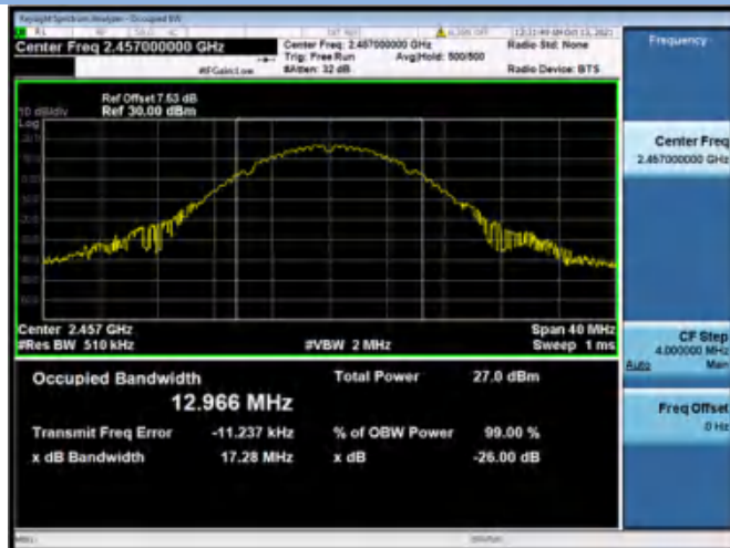
802.11b CHANNEL 10
