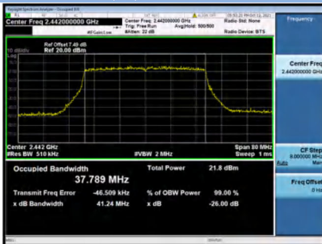
802.11ax-40 MHz(SU)CHANNEL 7
