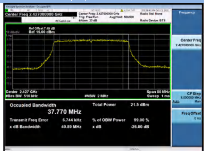
802.11ax-40 MHz(SU) CHANNEL 4
