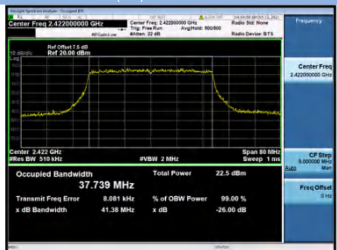
802.11ax-40 MHz(SU)CHANNEL 3
