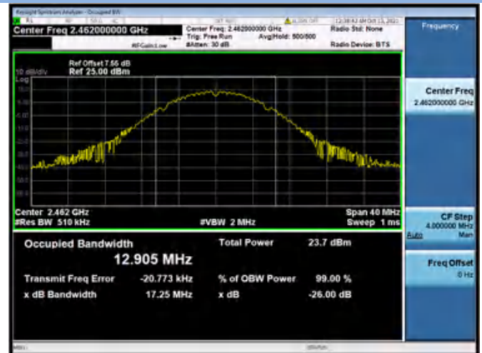
802.11b CHANNEL 11
