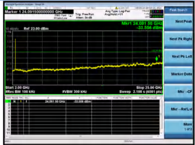
802.11g CHANNEL 10, SPURIOUS 2 GHz ~ 25 GHz
