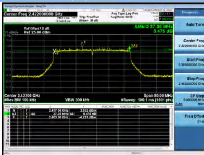
802.11ax-40 MHz(SU)CHANNEL 3
