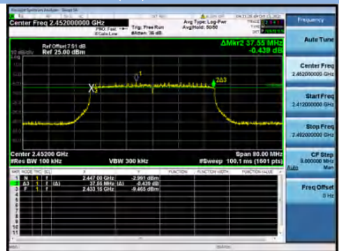
802.11ax-40 MHz(SU) CHANNEL 9
