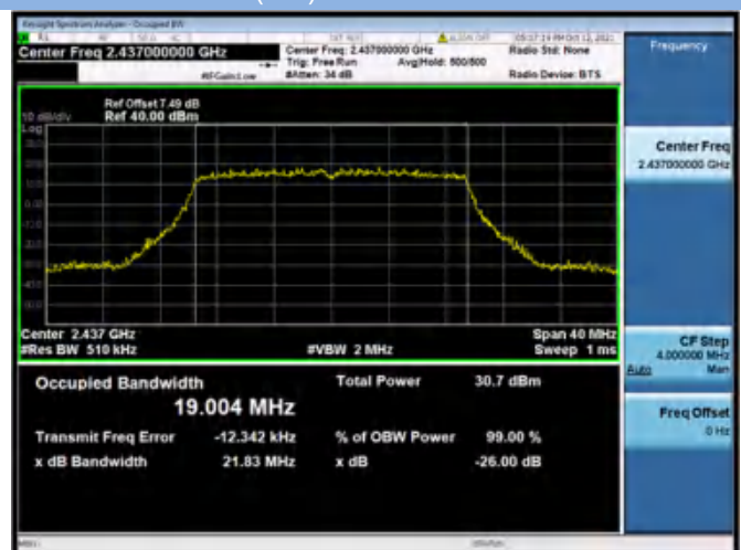
802.11ax-20 MHz(SU) CHANNEL 6
