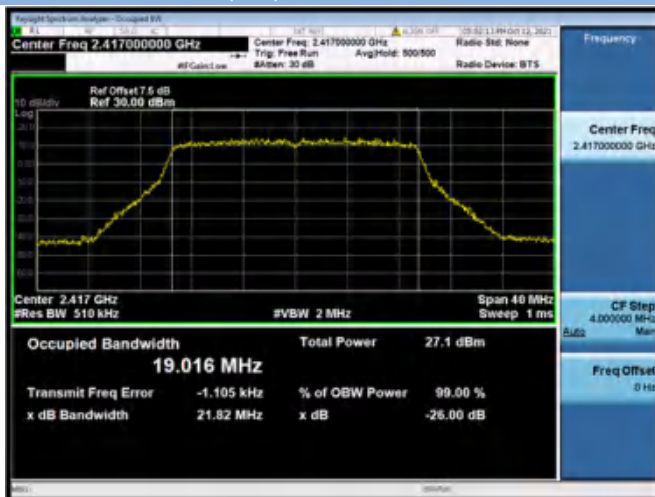
802.11ax-20 MHz(SU)CHANNEL 2
