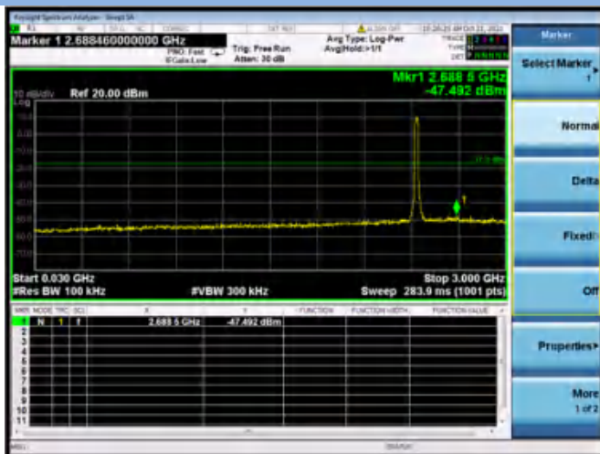
802.11ax-20(SU) CHANNEL 6, SPURIOUS 30 MHz ~ 3 GHz
