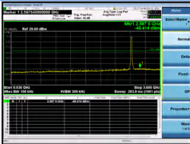
802.11ax-20(SU) CHANNEL 4, SPURIOUS 30 MHz ~ 3 GHz
