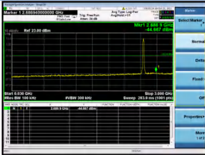
802.11g CHANNEL 10, SPURIOUS 30 MHz ~ 3 GHz
