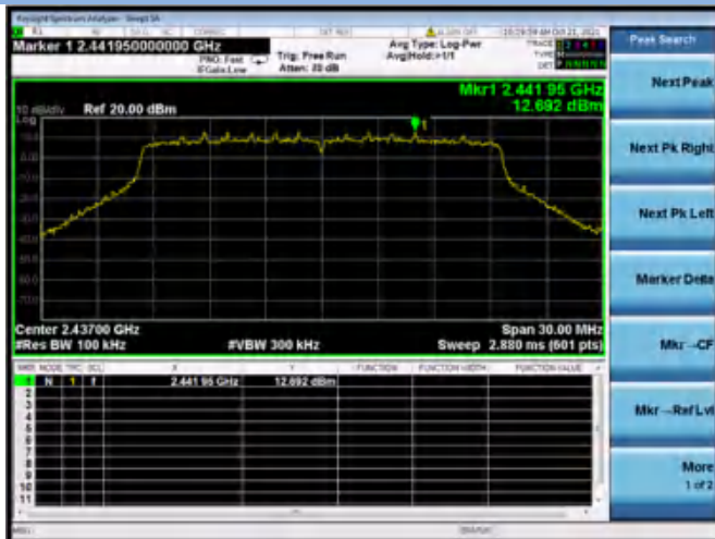
802.11ax-20(SU) CHANNEL 6 CARRIER LEVEL
