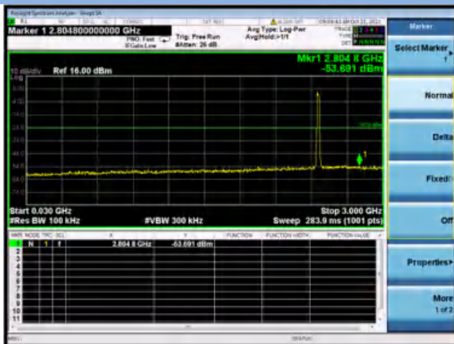
802.11g CHANNEL 11, SPURIOUS 30 MHz ~ 3 GHz
