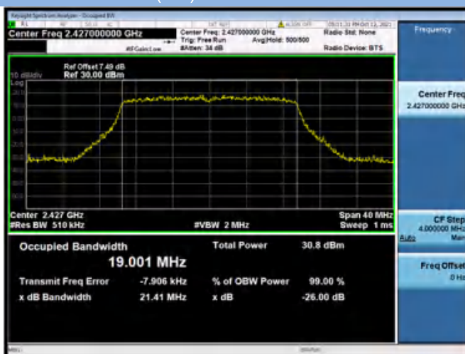
802.11ax-20 MH (SU)CHANNEL 4
