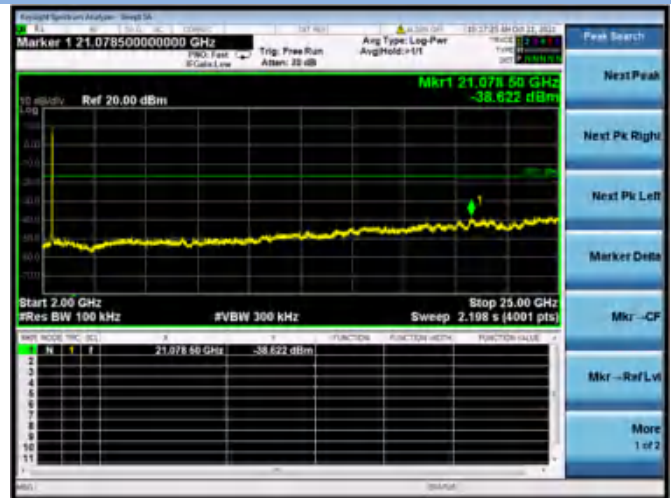
802.11ax-20(SU) CHANNEL 4, SPURIOUS 2 GHz ~ 25 GHz
