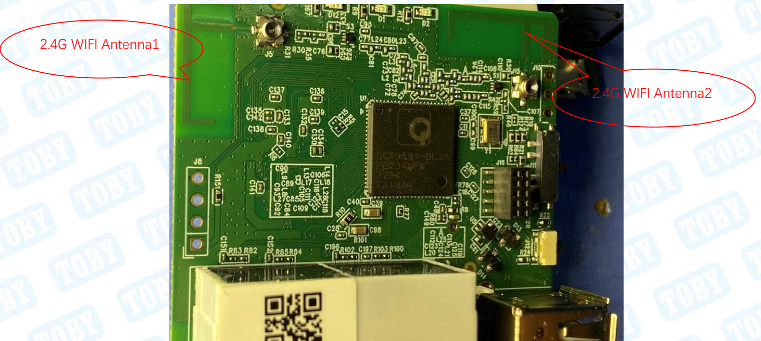
Photo 16 Appearance of PCB
