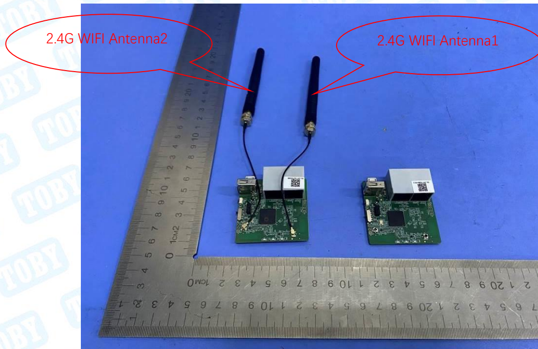
Photo 12 Internal of EUT
