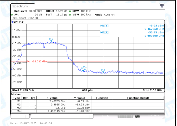
11N40MIMO-Ant2-2452-PASS
