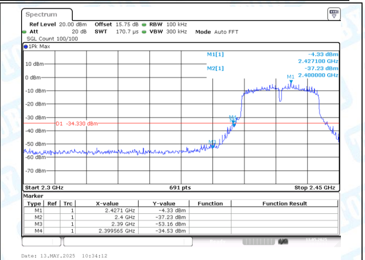
11N40MIMO-Ant2-2422-PASS
