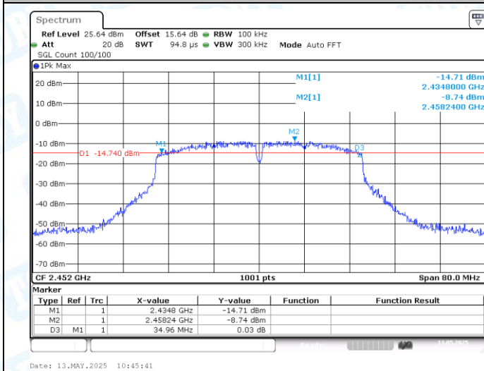
11N40MIMO-Ant1-2452-PASS
