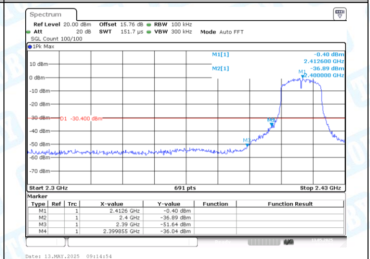
11G-CDD-Ant2-2412-PASS
