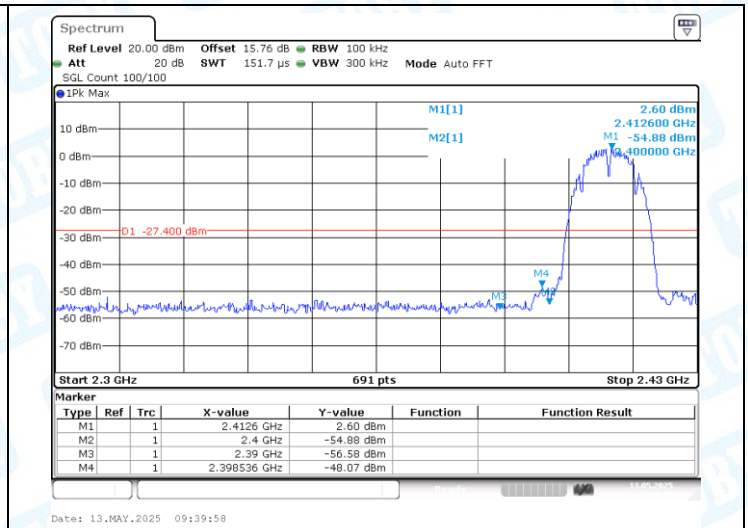
11B-CDD-Ant2-2412-PASS
