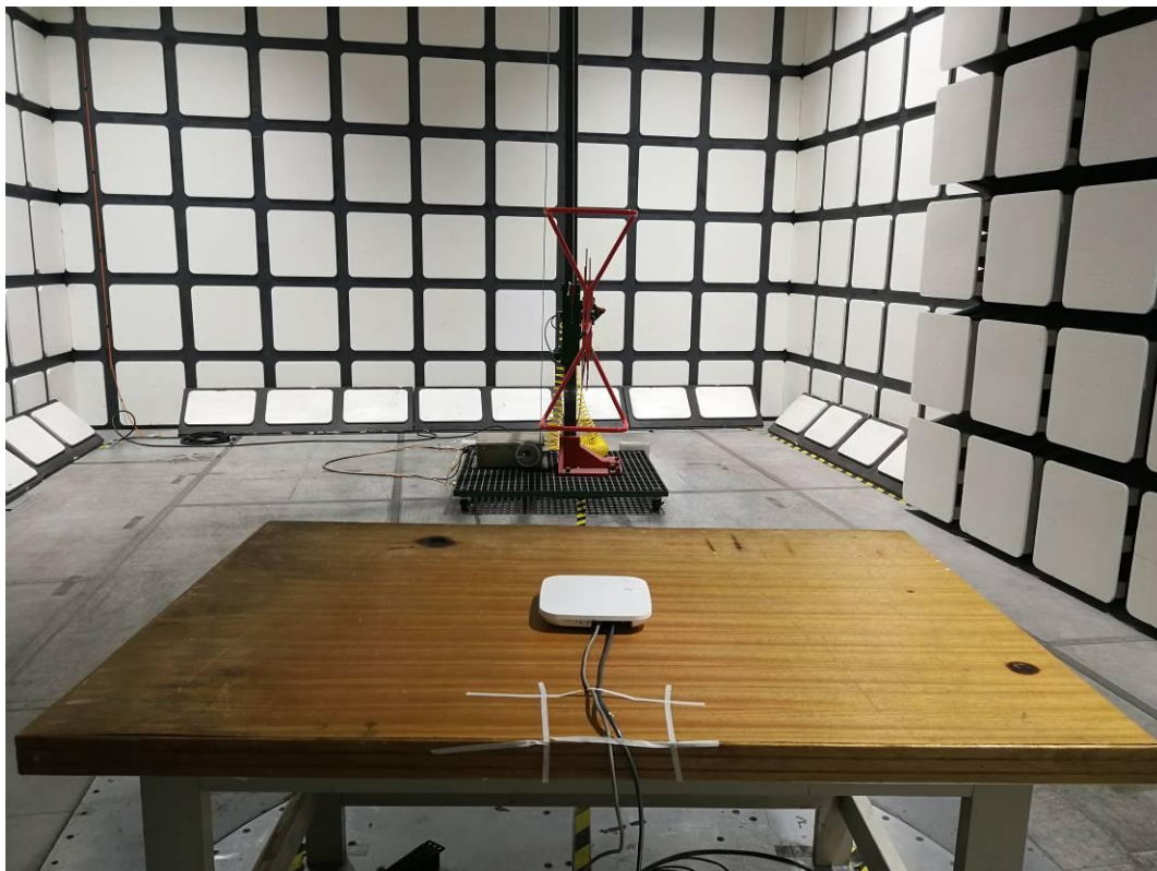
Radiated Emissions View (Below 1 GHz, for POE)
