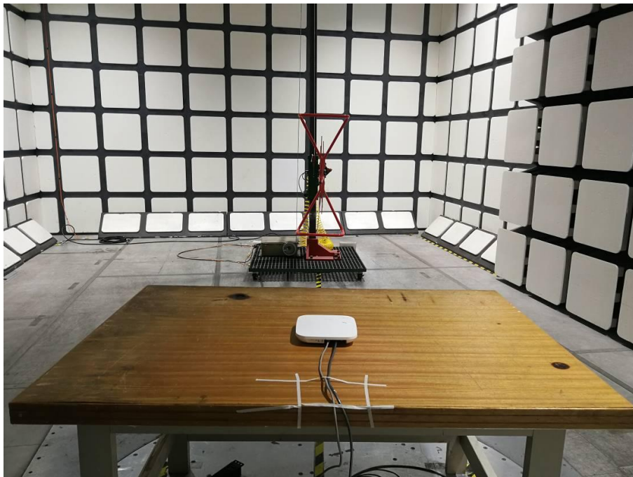
Radiated Emissions View (Below 1 GHz, for POE)
