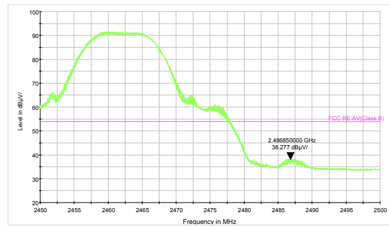
802.11g, Channel No.: 11 - PK
