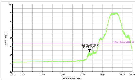
802.11g, Channel No.: 1 - PK
