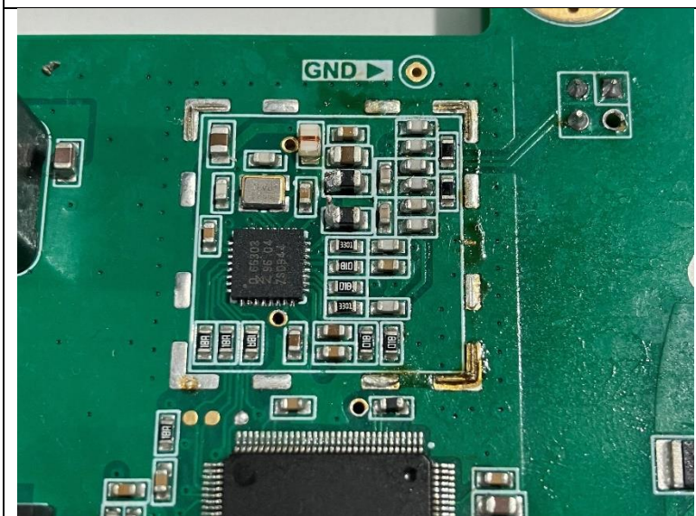
RFID Circuit - Can Removed
