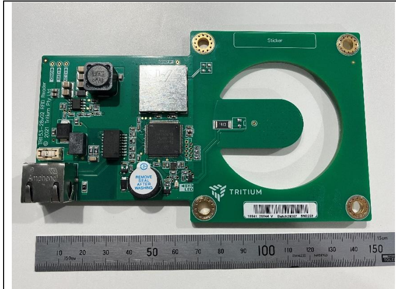
Circuit Board
