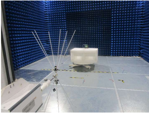
Biconical Antenna (30 – 300 MHz)
