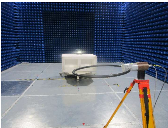
Antenna Ground-Parallel
