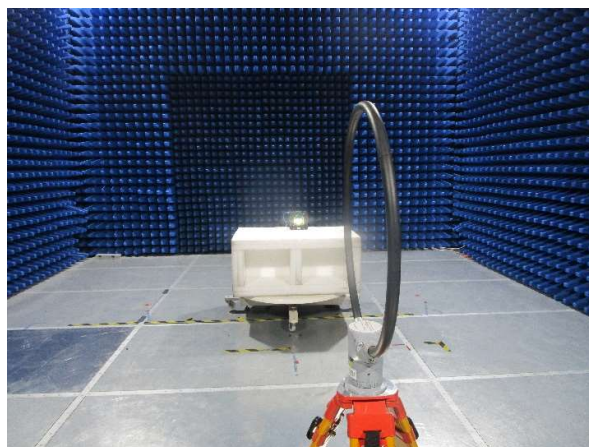
Antenna Perpendicular (9 kHz to 30 MHz)
