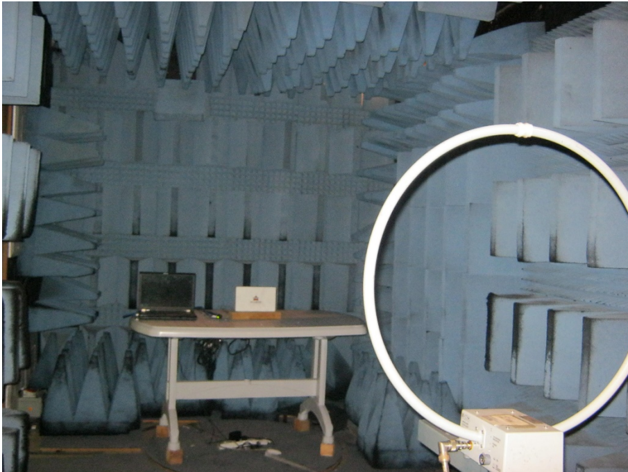
Radiated Emission Test, 0.009-30MHz band
