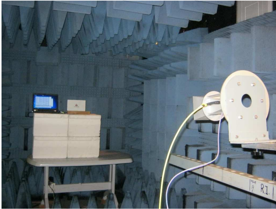
Figure 5. Radiated Emission Test, 1000-18,000MHz band
