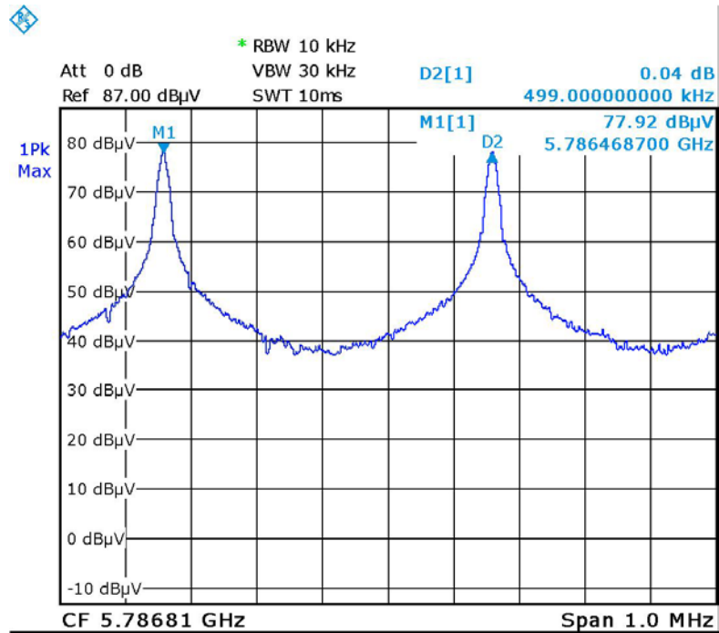
Figure 33. Channel Frequency Separation
