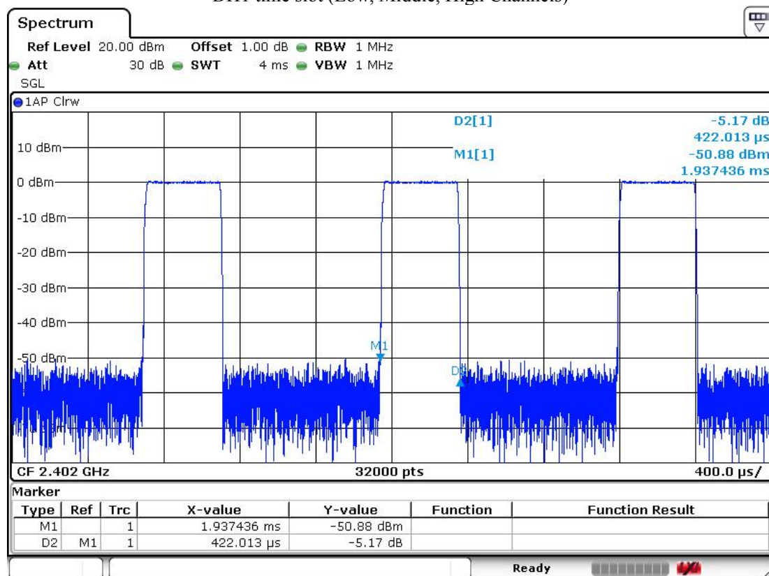
DH1 time slot (Low, Middle, High Channels)
