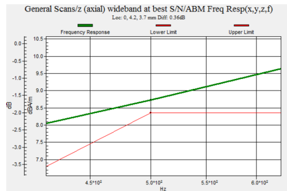
Fig 7.4 GSM1900 Ch661
