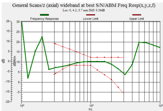
Fig 7.3 GSM1900 Ch661
