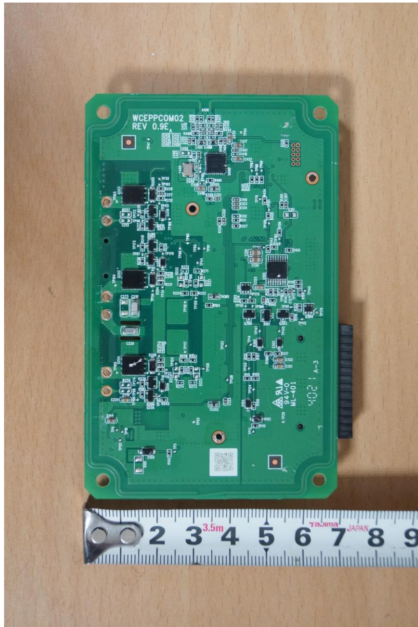
< Main board bottom view #2 >
