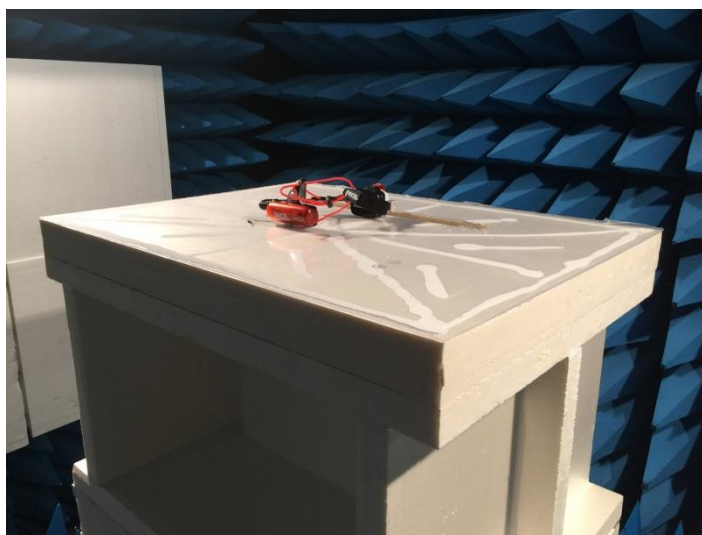
Test setup in anechoic chamber for configuration2:
