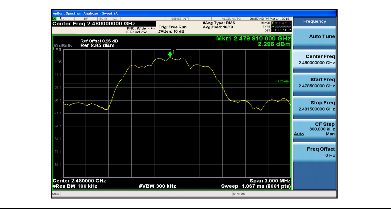
RF Conducted Spurious Emissions_2DH5_2480
