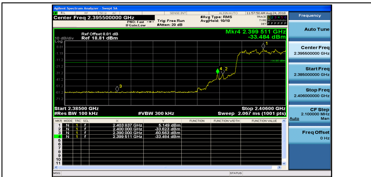
Band-edge for RF Conducted Emissions_3DH5_2402_Hopping Off
