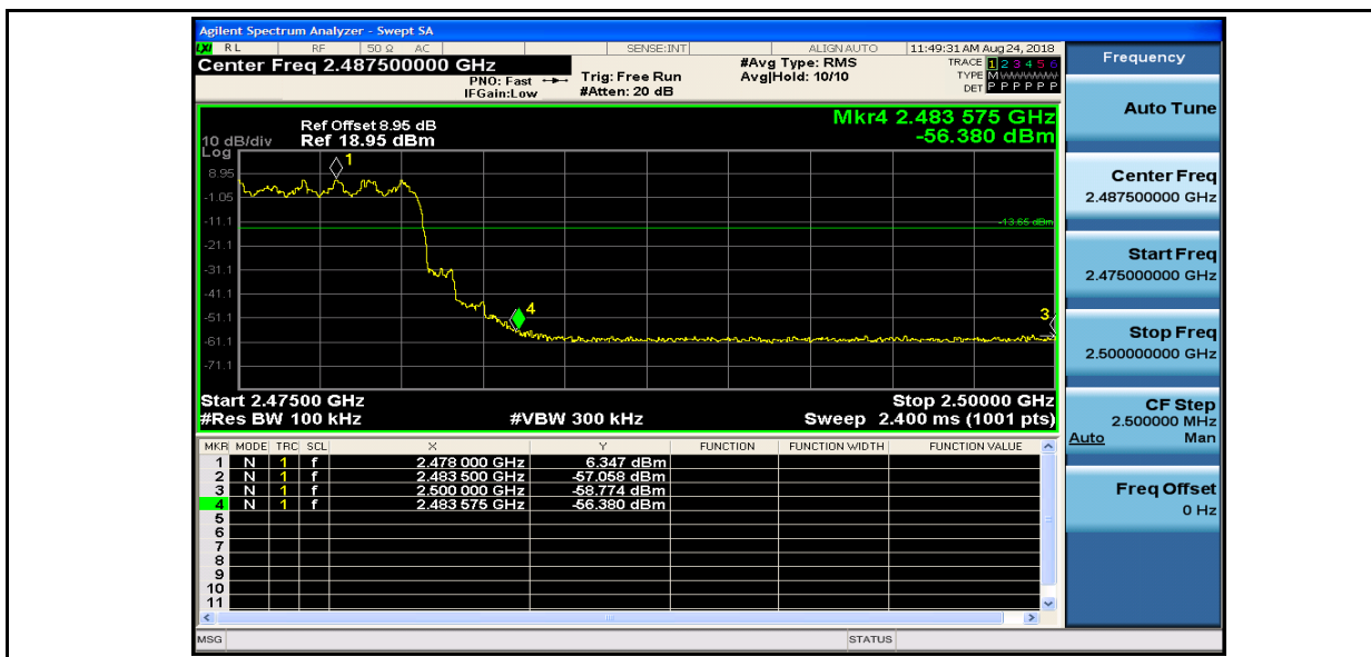
Band-edge for RF Conducted Emissions_2DH5_2480_Hopping Off
