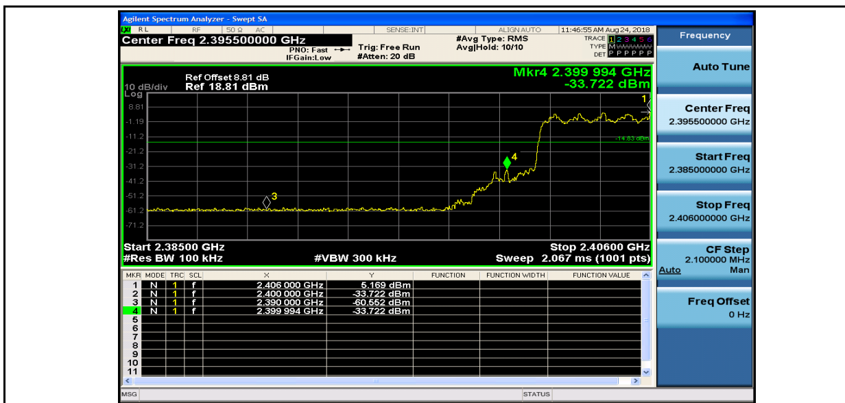
Band-edge for RF Conducted Emissions_2DH5_2402_Hopping Off
