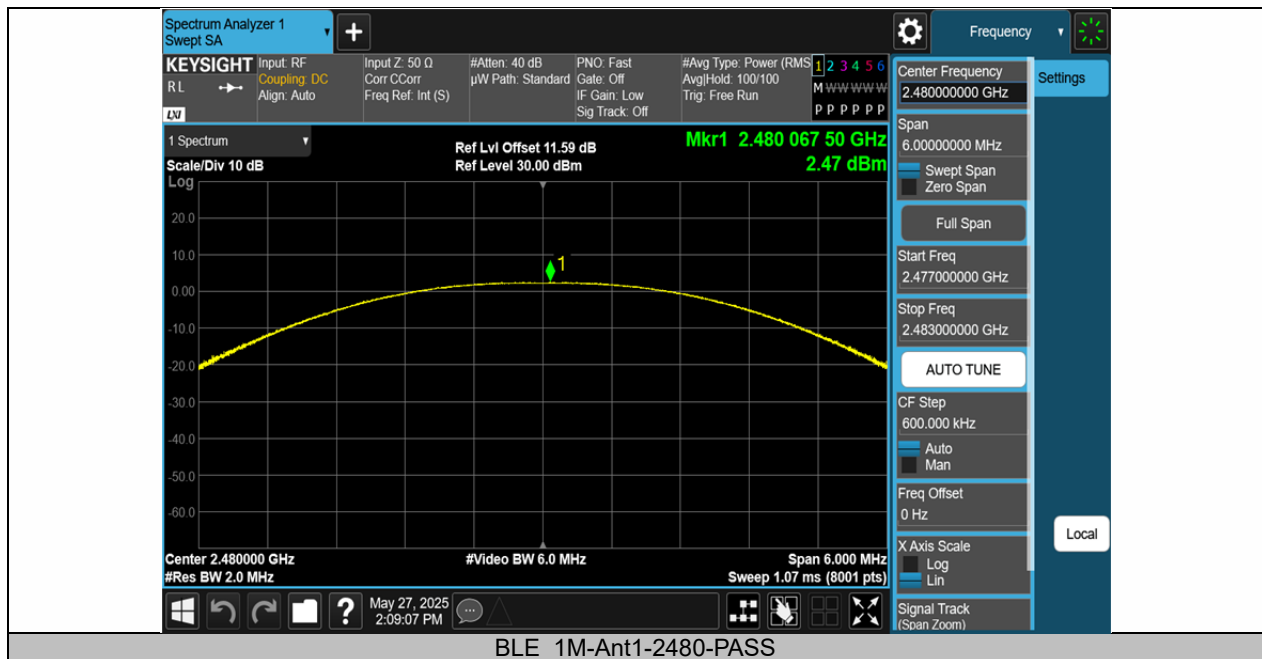
BLE_1M-Ant1-2480-PASS
