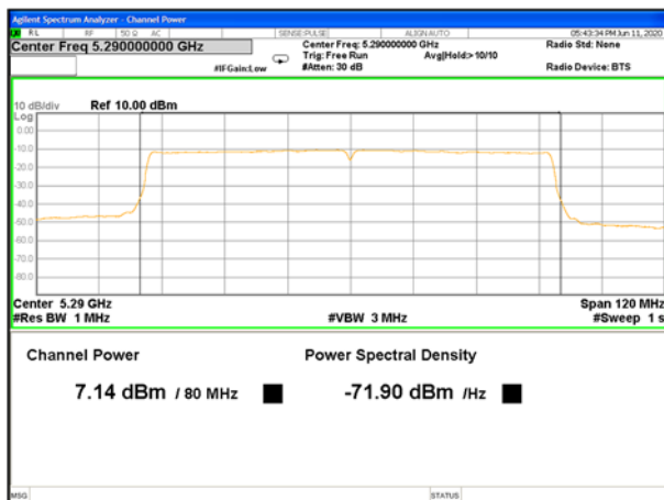
5290MHz_AV_Ant B
