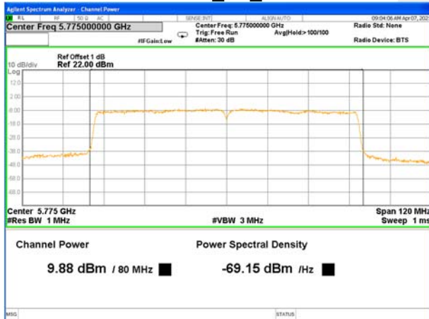
5775MHz_AV_Ant B
