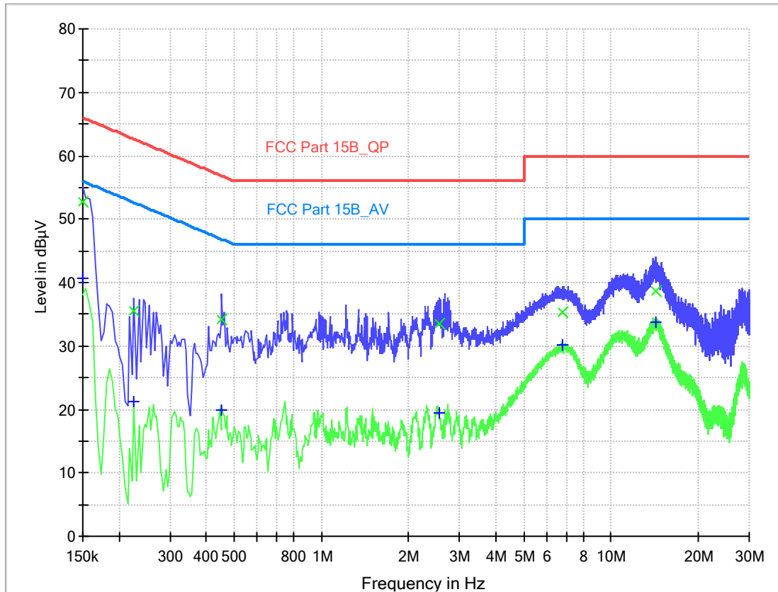
Plots No. 8: AC Mains Conducted Emission _ AC 120V/60Hz _ High Channel _ Neutral
