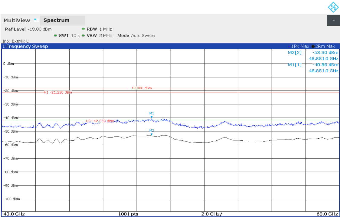
Plots No. 4: 40 GHz to 60 GHz, Horizontal / Vertical Polarization
