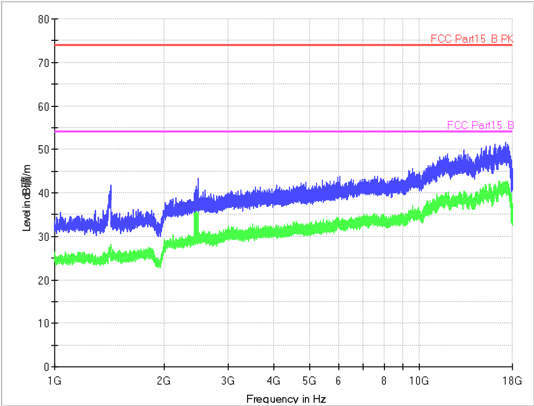
Plots No. 2: 1 GHz to 18 GHz, Horizontal / Vertical Polarization
