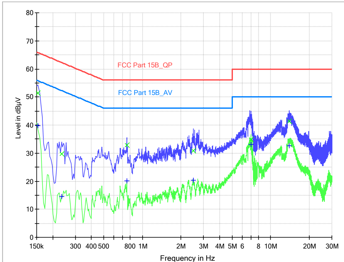
Plots No. 7: AC Mains Conducted Emission _ AC 120V/60Hz _ High Channel _ Line
