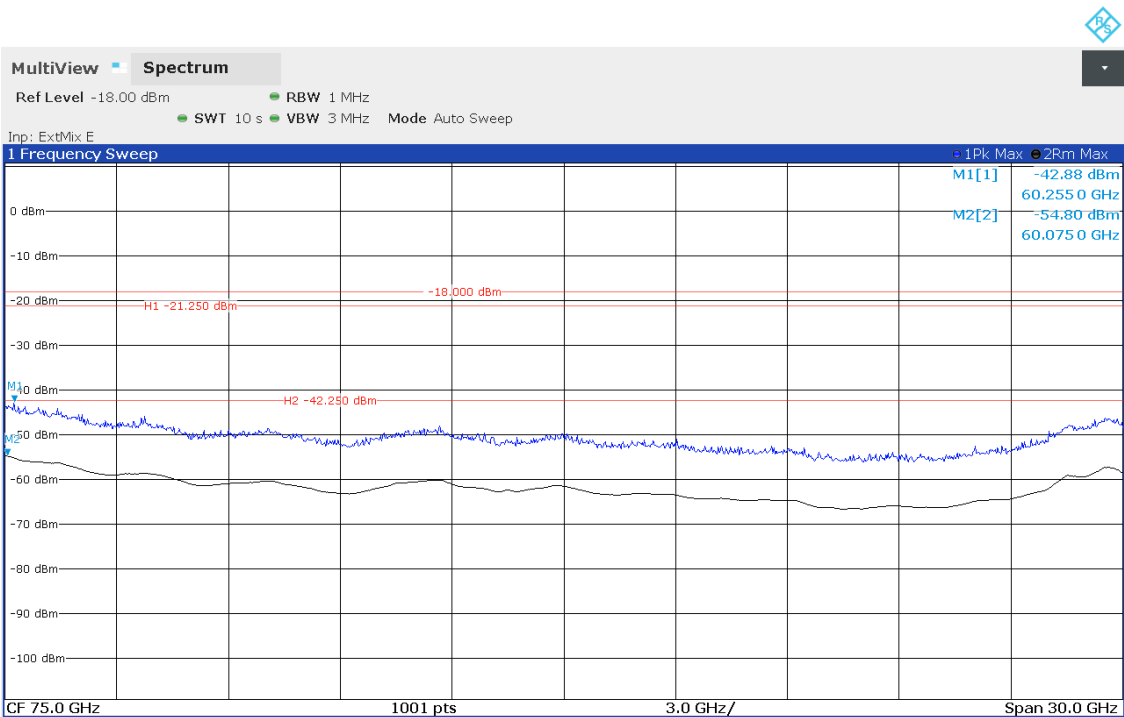
Plots No. 5: 60 GHz to 90 GHz, Horizontal / Vertical Polarization
