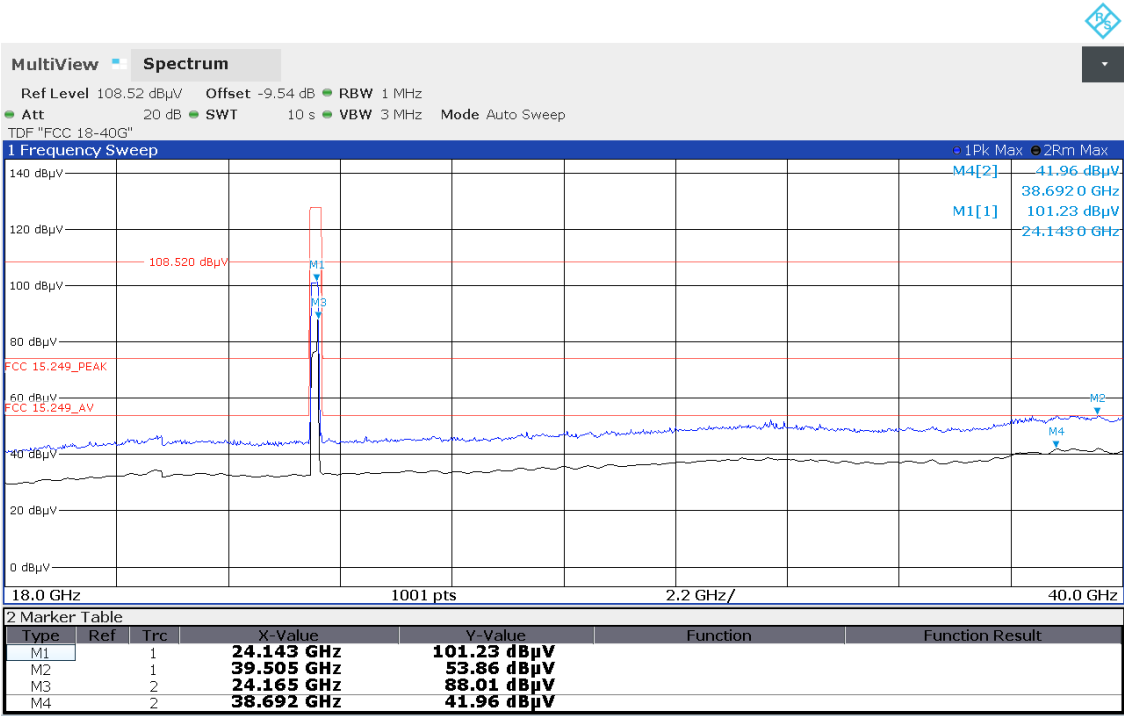
Plots No. 3: 18 GHz to 40 GHz, Horizontal / Vertical Polarization
