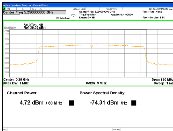
5290MHz_AV_Ant A
