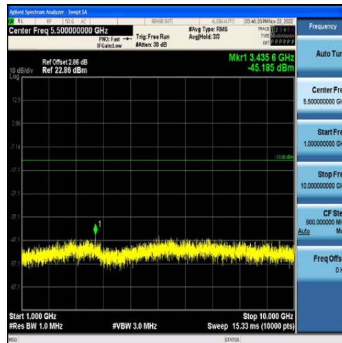
Band12-3MHz-16QAM-23095-15RB#0-Range2:1000~10000MHz
