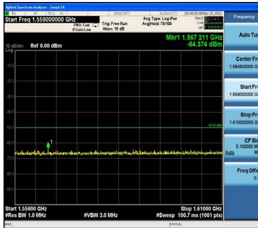
Band13-10MHz-QPSK-23230-50RB#0-Range3:1559~1610MHz
