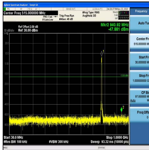
Band13-5MHz-16QAM-23205-25RB#0-Range1:30~1000MHz
