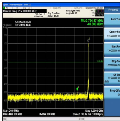
Band5-3MHz-QPSK-20635-15RB#0-Range1:30~1000MHz
