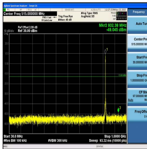
Band5-3MHz-16QAM-20415-15RB#0-Range1:30~1000MHz
