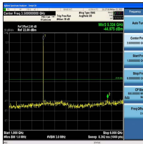
Band7-5MHz-16QAM-20775-25RB#0-Range2:1000~6000MHz
