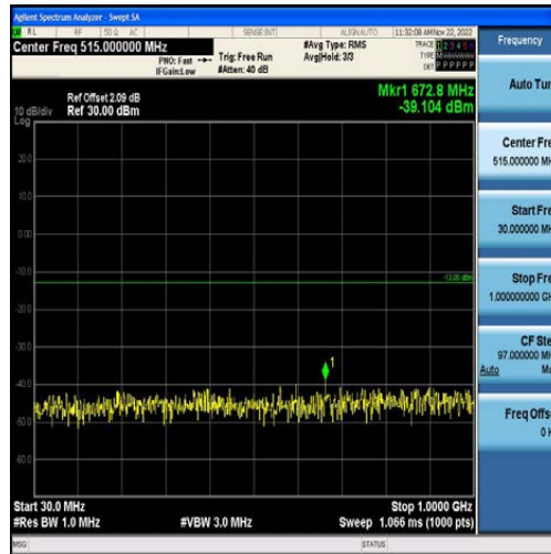
Band4-15MHz-16QAM-20175-75RB#0-Range1:30~1000MHz
