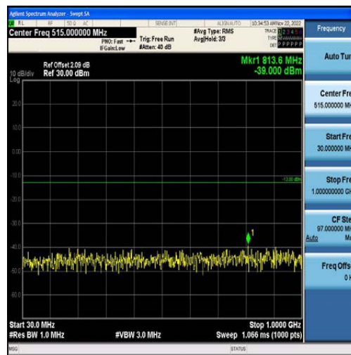
Band4-10MHz-16QAM-20000-50RB#0-Range1:30~1000MHz
