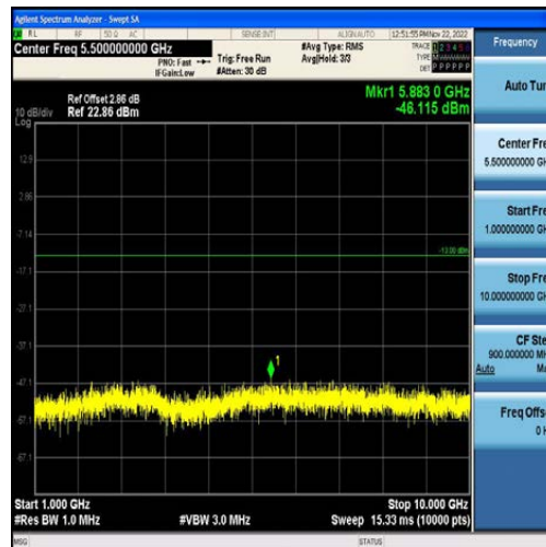
Band5-10MHz-16QAM-20525-50RB#0-Range2:1000~10000MHz
