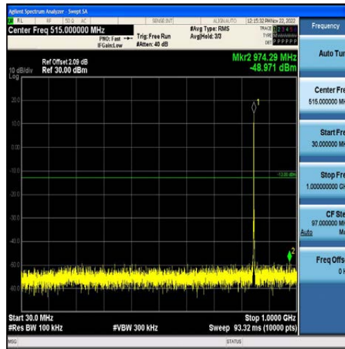
Band5-1.4MHz-QPSK-20643-6RB#0-Range1:30~1000MHz
