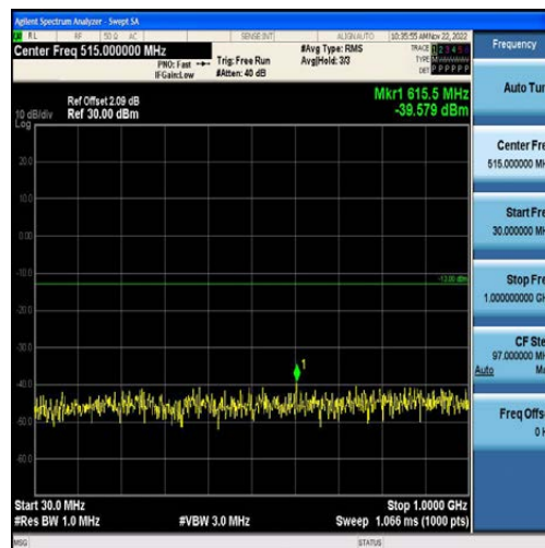
Band4-10MHz-16QAM-20350-50RB#0-Range1:30~1000MHz
