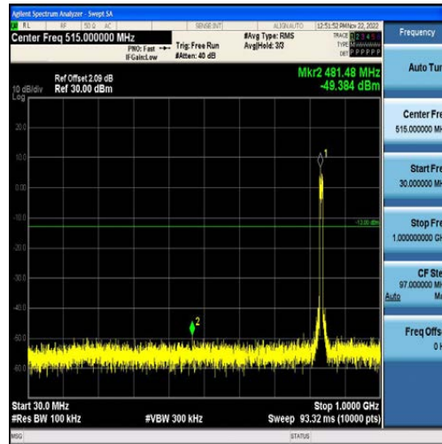
Band5-10MHz-16QAM-20525-50RB#0-Range1:30~1000MHz
