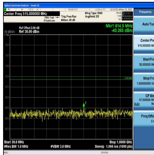
Band4-5MHz-16QAM-20375-25RB#0-Range1:30~1000MHz
