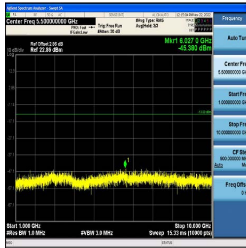
Band5-1.4MHz-QPSK-20525-6RB#0-Range2:1000~10000MHz
