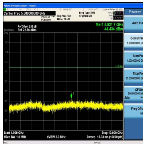
Band5-1.4MHz-QPSK-20407-6RB#0-Range2:1000~10000MHz
