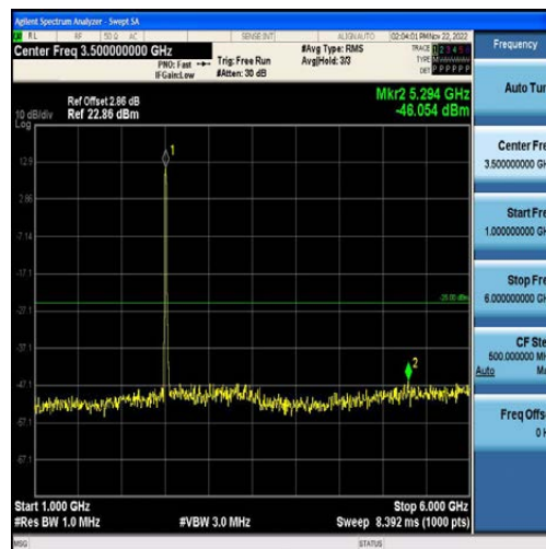
Band7-15MHz-16QAM-20825-75RB#0-Range2:1000~6000MHz
