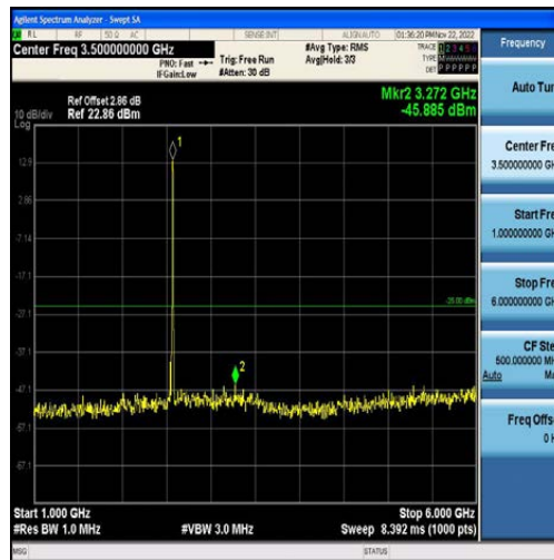
Band7-5MHz-16QAM-21425-25RB#0-Range2:1000~6000MHz
