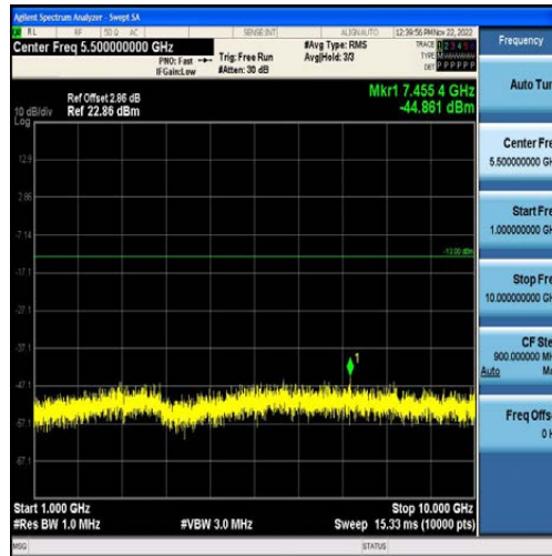
Band5-5MHz-QPSK-20625-25RB#0-Range2:1000~10000MHz
