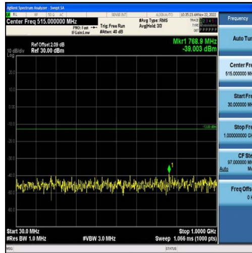
Band4-10MHz-16QAM-20175-50RB#0-Range1:30~1000MHz
