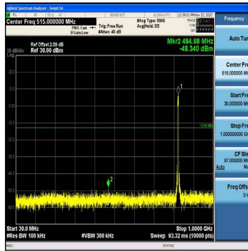
Band5-5MHz-16QAM-20425-25RB#0-Range1:30~1000MHz
