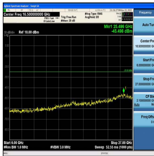
Band7-5MHz-16QAM-21425-25RB#0-Range3:6000~27000MHz
