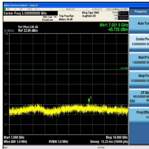
Band5-10MHz-QPSK-20450-50RB#0-Range2:1000~10000MHz
