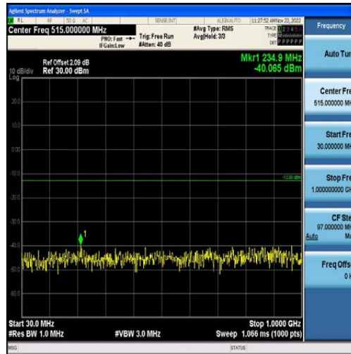
Band4-15MHz-QPSK-20025-75RB#0-Range1:30~1000MHz
