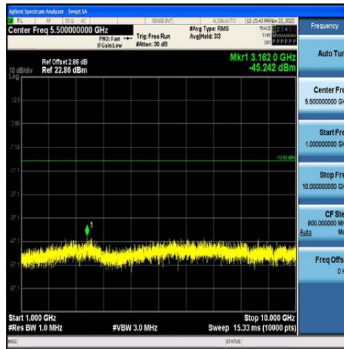
Band5-1.4MHz-16QAM-20643-6RB#0-Range2:1000~10000MHz
