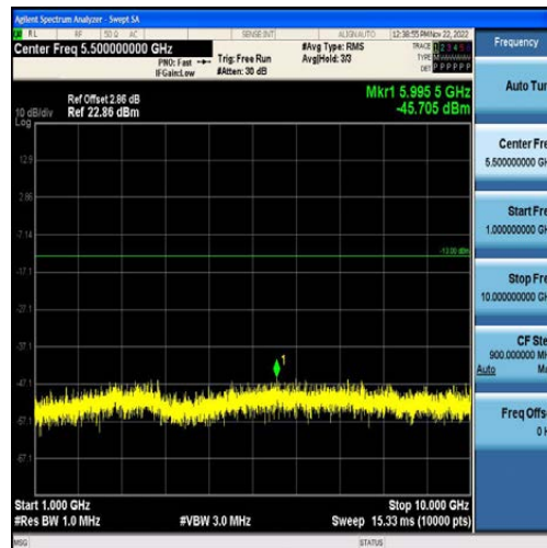
Band5-5MHz-QPSK-20425-25RB#0-Range2:1000~10000MHz
