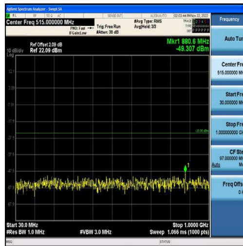
Band7-15MHz-QPSK-20825-75RB#0-Range1:30~1000MHz
