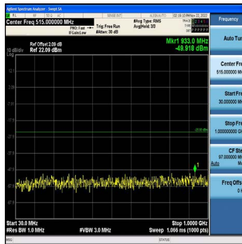
Band7-15MHz-QPSK-21375-75RB#0-Range1:30~1000MHz
