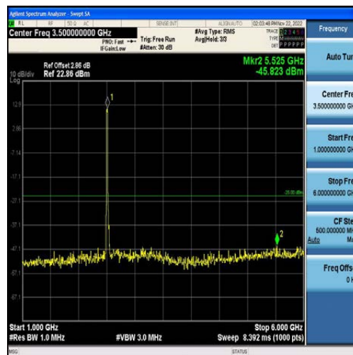
Band7-15MHz-QPSK-20825-75RB#0-Range2:1000~6000MHz
