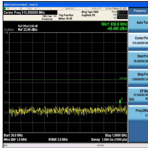
Band7-5MHz-16QAM-21425-25RB#0-Range1:30~1000MHz
