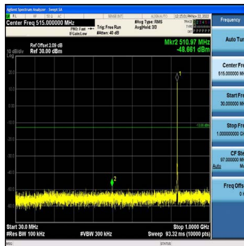
Band5-1.4MHz-QPSK-20525-6RB#0-Range1:30~1000MHz
