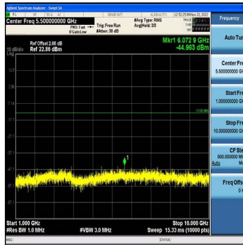
Band5-10MHz-16QAM-20600-50RB#0-Range2:1000~10000MHz
