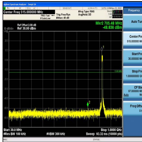
Band5-10MHz-QPSK-20450-50RB#0-Range1:30~1000MHz
