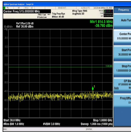
Band4-5MHz-QPSK-20375-25RB#0-Range1:30~1000MHz
