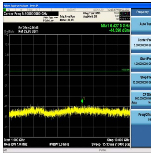
Band5-1.4MHz-QPSK-20643-6RB#0-Range2:1000~10000MHz
