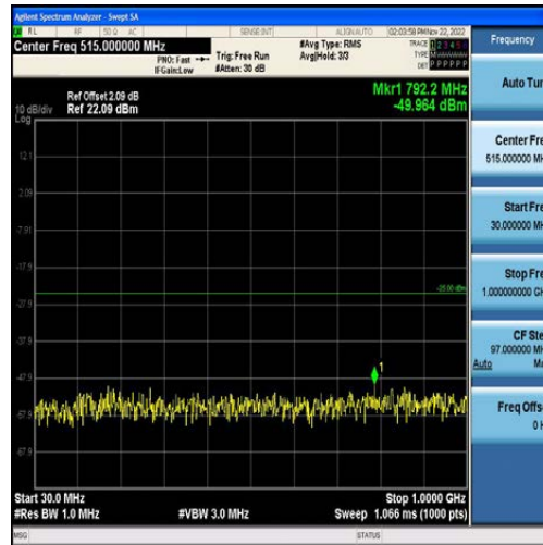
Band7-15MHz-16QAM-20825-75RB#0-Range1:30~1000MHz
