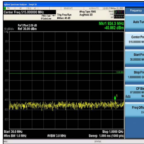
Band4-20MHz-QPSK-20050-100RB#0-Range1:30~1000MHz
