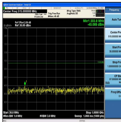
Band4-20MHz-16QAM-20300-100RB#0-Range1:30~1000MHz
