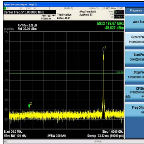
Band5-5MHz-QPSK-20425-25RB#0-Range1:30~1000MHz
