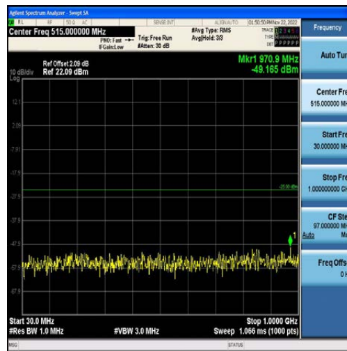
Band7-10MHz-16QAM-20800-50RB#0-Range1:30~1000MHz
