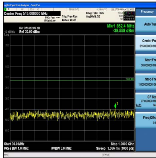
Band4-15MHz-16QAM-20025-75RB#0-Range1:30~1000MHz
