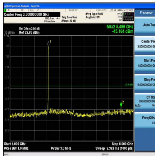
Band7-15MHz-QPSK-21375-75RB#0-Range2:1000~6000MHz
