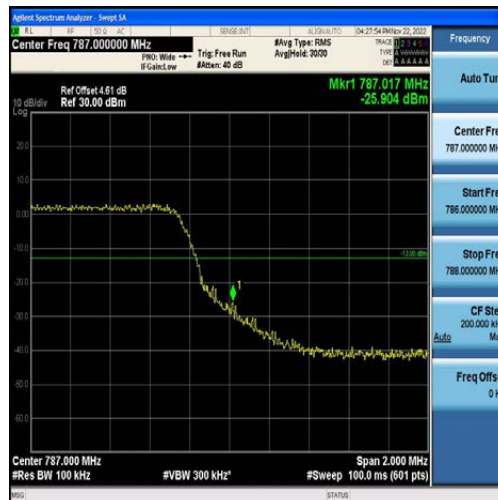
Band13-5MHz-QPSK-23255-25RB#0
