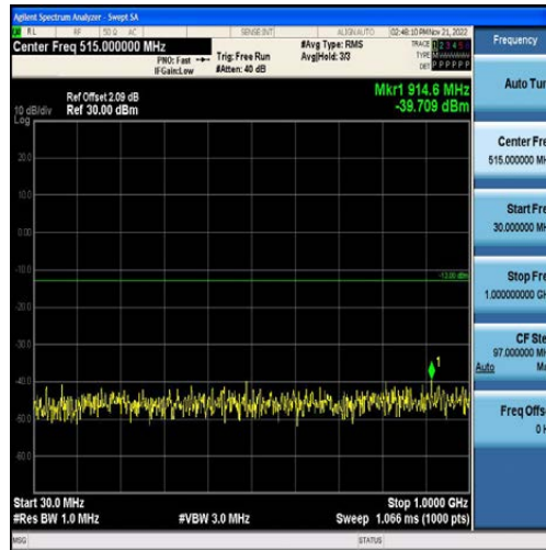
Band2-3MHz-16QAM-18900-15RB#0-Range1:30~1000MHz
