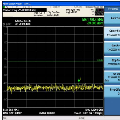
Band4-1.4MHz-16QAM-20175-6RB#0-Range1:30~1000MHz
