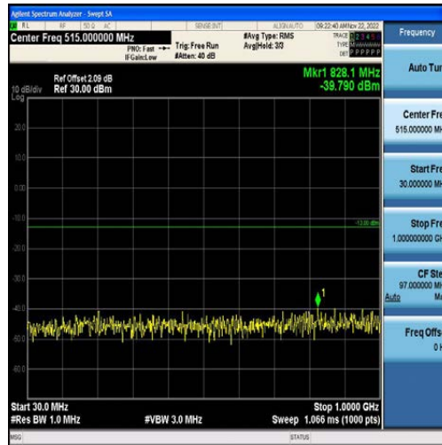
Band2-10MHz-16QAM-18900-50RB#0-Range1:30~1000MHz
