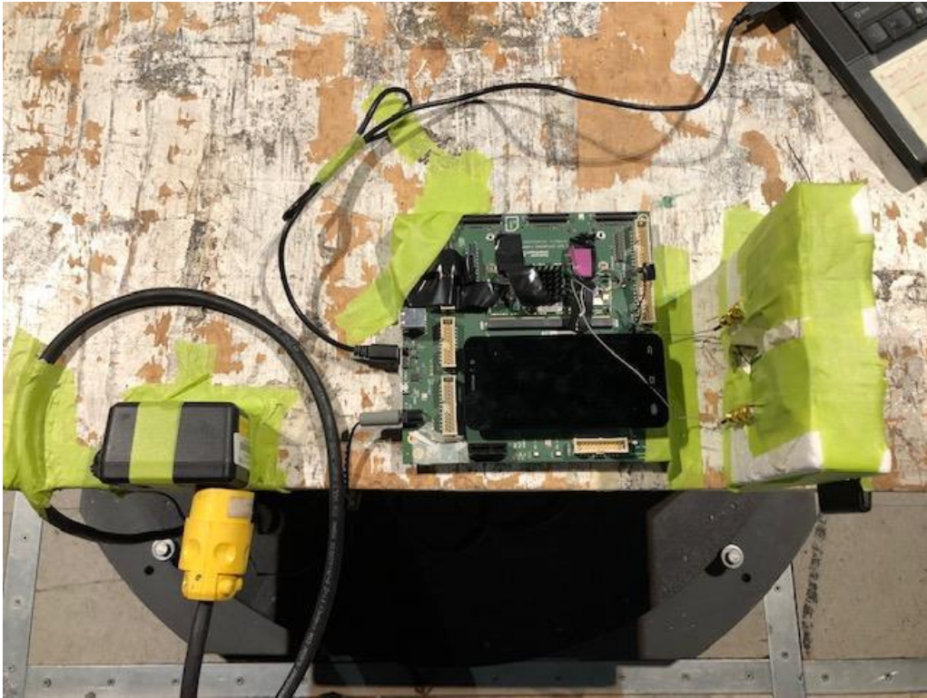
Radiated Emissions 3m SAC Setup – Photo1
