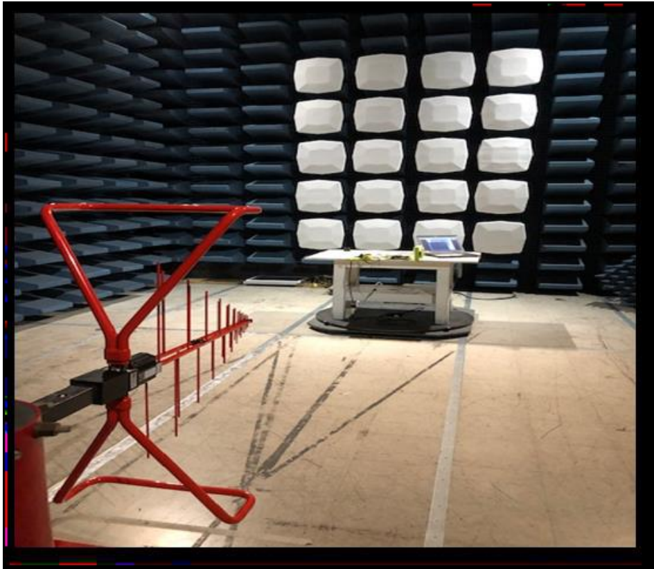
Radiated Emissions 3m SAC 30 – 1000MHz
