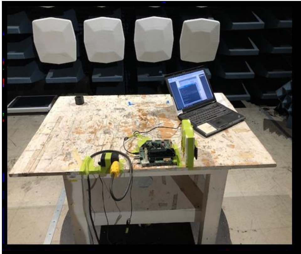
Radiated Emissions 3m SAC Setup – Photo3
