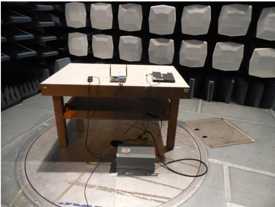
AC Conducted Emissions 3m SAC
