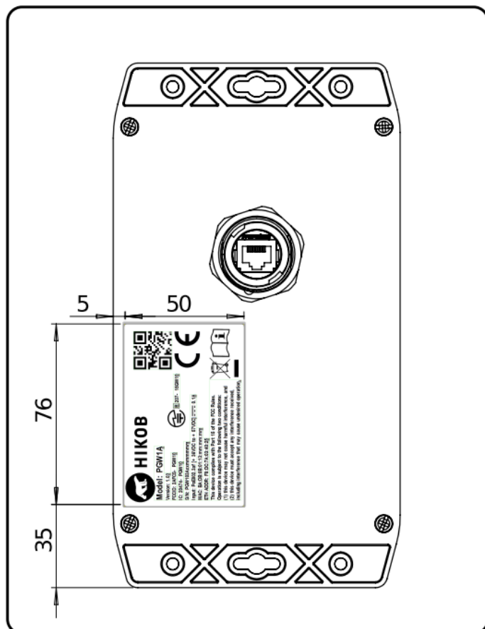
Figure 18: HIKOB GATEWAY - PGW1C casing label
