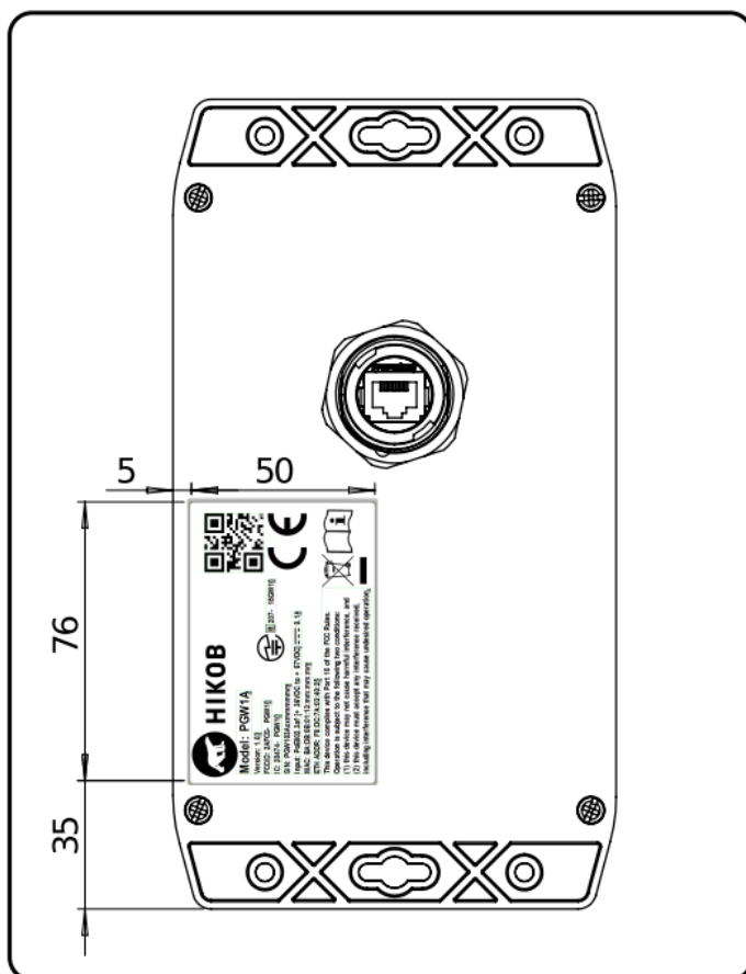
Figure 10: HIKOB GATEWAY - PGW1A casing label
