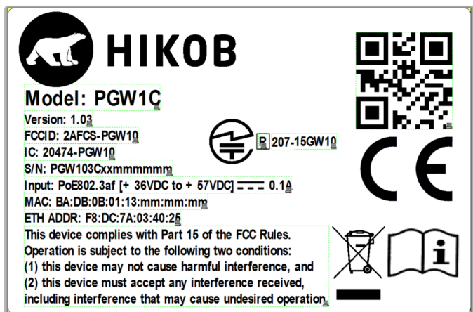
Figure 17: HIKOB GATEWAY - PGW1C casing label
