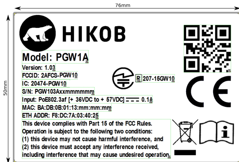
Figure 6: Label on casing
