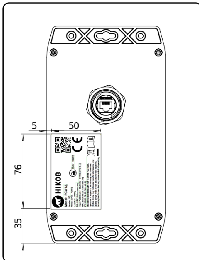
Figure 14: HIKOB GATEWAY - PGW1B casing label
