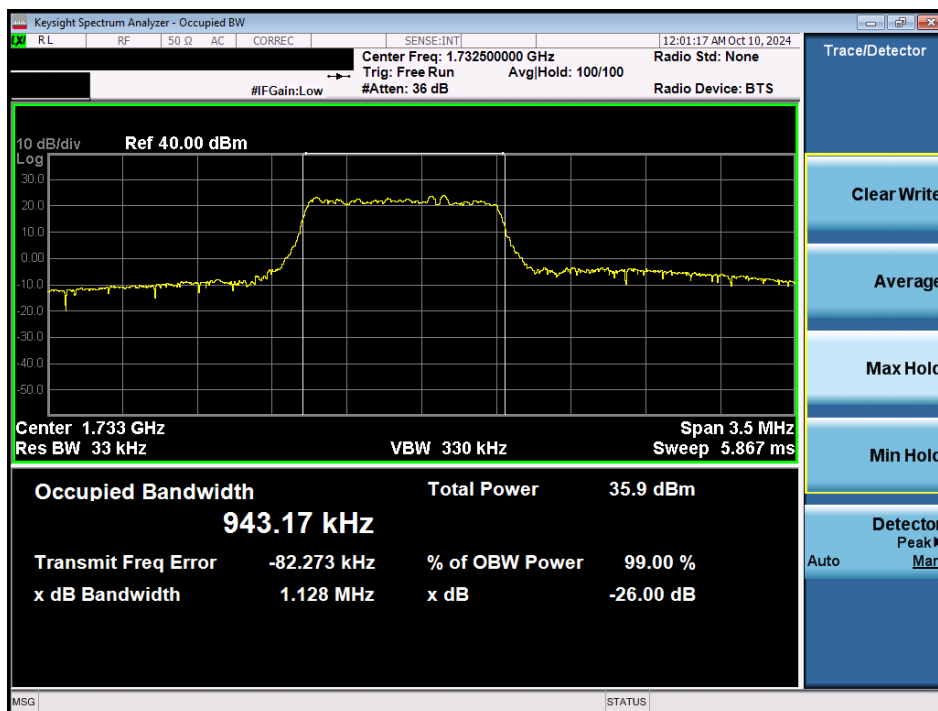
Plot 7-2. Occupied Bandwidth Plot (LTE Band 4 - 1.4MHz 16-QAM - Full RB)
