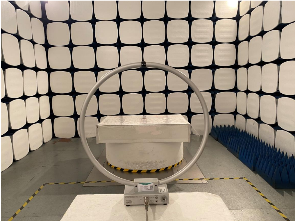
Radiated Emission 9kHz-30MHz
