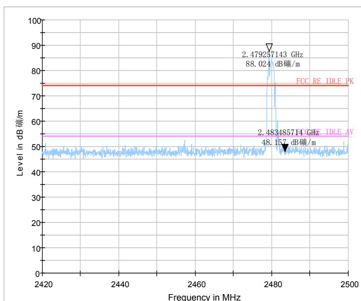
Fig.50 Radiated emission (Power): \pi/4 DQPSK, high channel
