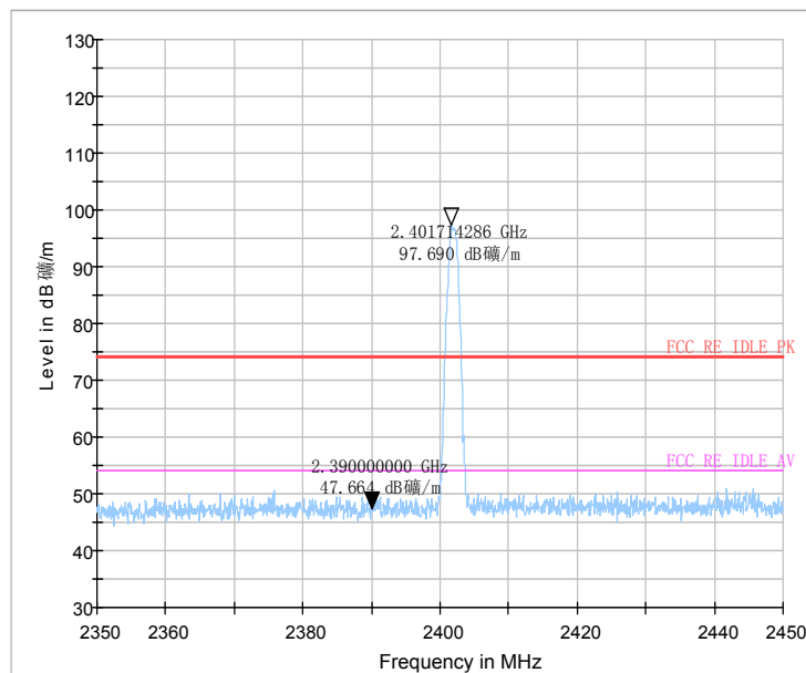
Fig.43 Radiated emission (Power): GFSK, low channel
