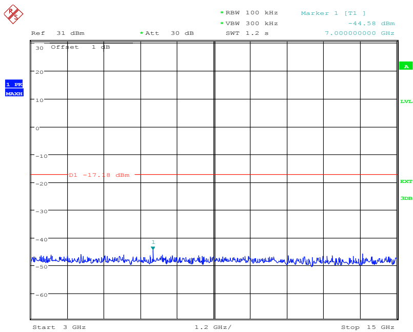
(Plot 4.9.1 A1: Channel 00: 2402MHz @ GFSK)
