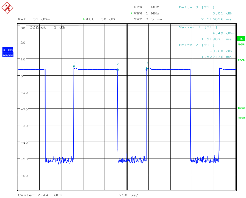
(Plot 4.8.1.A: Channel 39: 2441MHz @ GFSK @ DH1)
