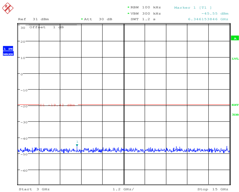
(Plot 4.9.2 A1: Channel 00: 2402MHz @ 8DPSK)
