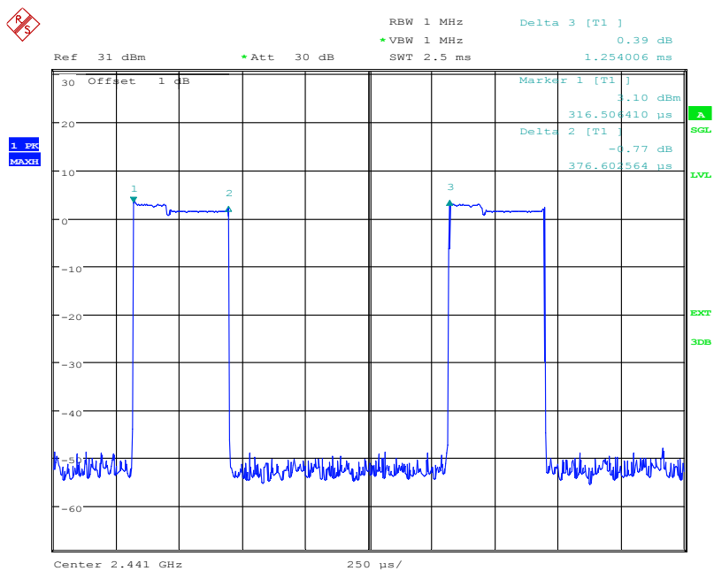
(Plot 4.8.1.C: Channel 39: 2441MHz @ GFSK @ DH1)
