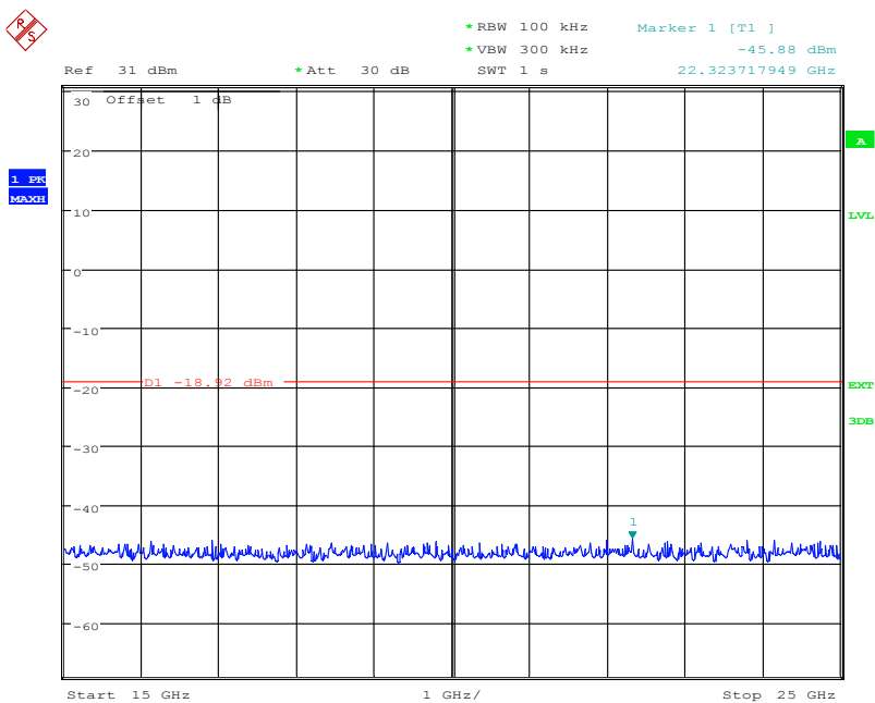
(Plot 4.9.2 B2: Channel 39: 2441MHz @ @ 8DPSK)
