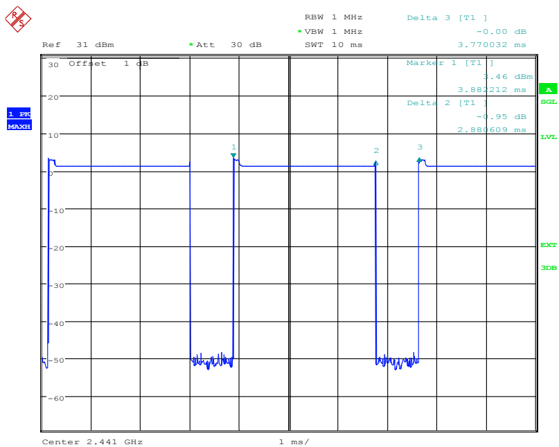
(Plot 4.8.2.B: Channel 39: 2441MHz @ 8DPSK @ DH3)
