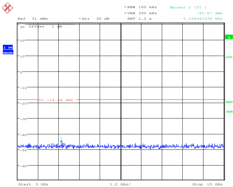
(Plot 4.9.2 C1: Channel 78: 2480MHz @ @ 8DPSK)
