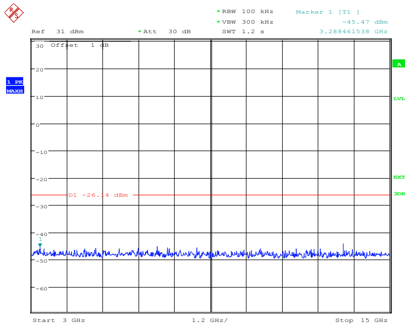
(Plot 4.6.1 C1: Channel 39: 2480MHz @ GFSK)
