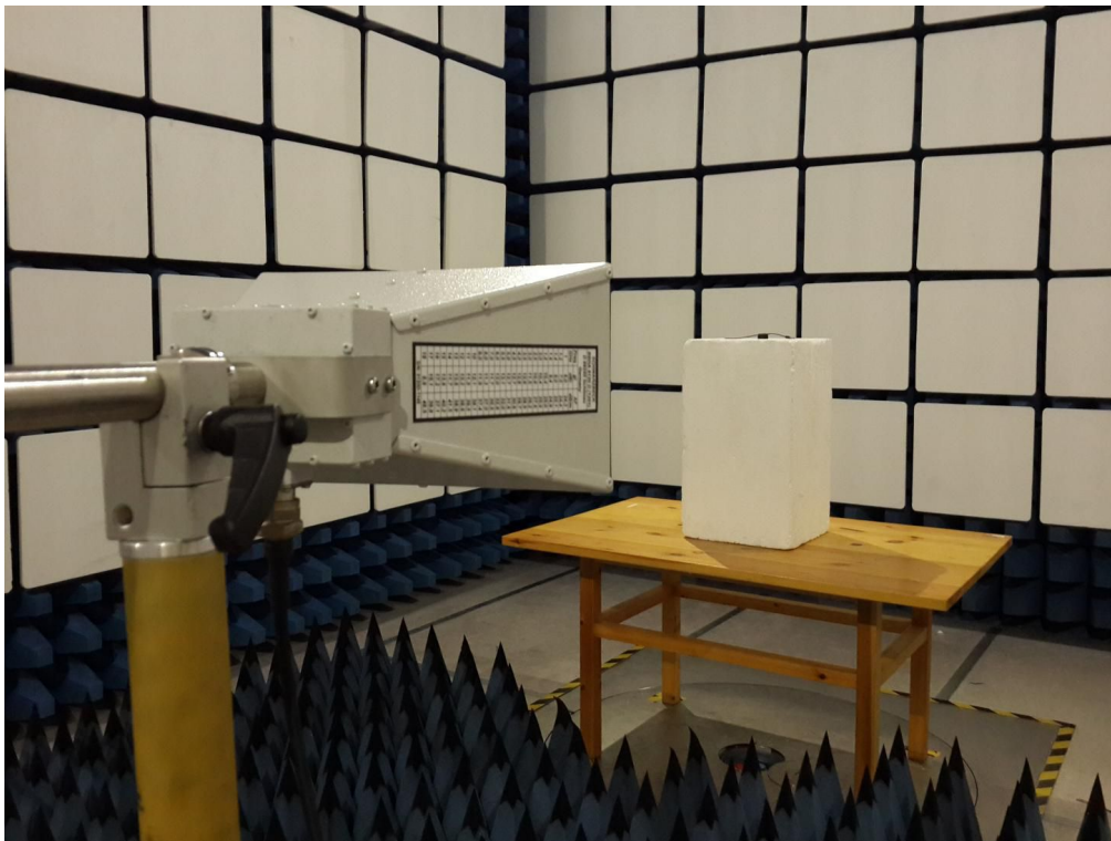
Above 1GHz-1
