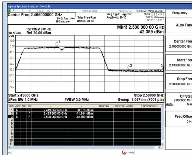
Channel 9 / 2452 MHz – Peak
