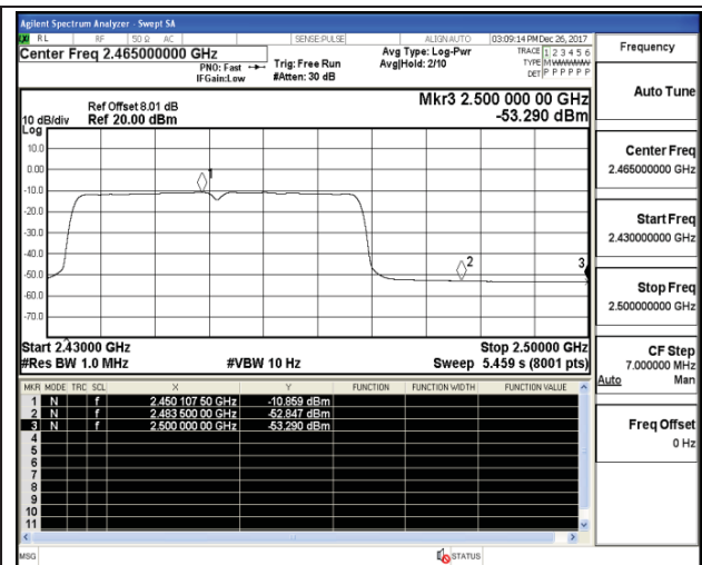
Channel 9 / 2452 MHz – Average
