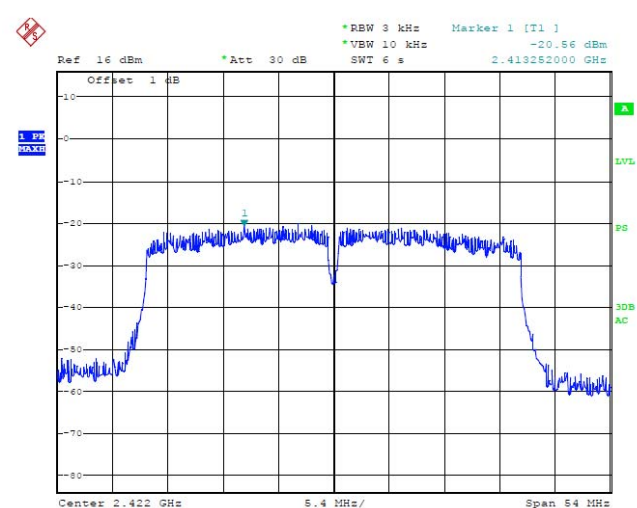
CH3 / 2422 MHz
