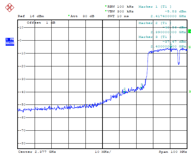
Ch3 / 2422 MHz
