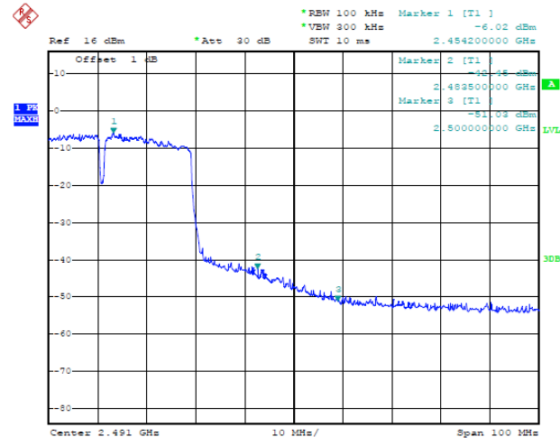
Ch9 / 2452 MHz
