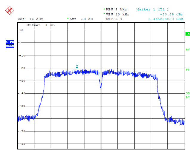
CH9 / 2452 MHz
