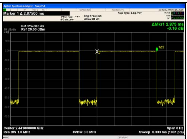
GFSK - Mid CH 2441
